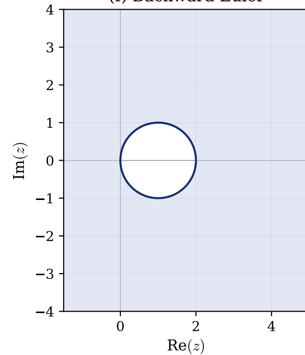
(f) Backward Euler
