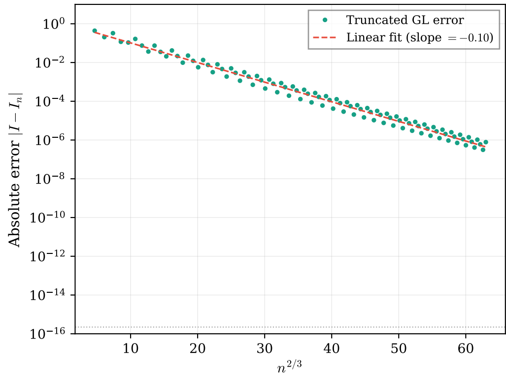
(b) Truncated GL: O(e^{-Cn^{2/3}})
