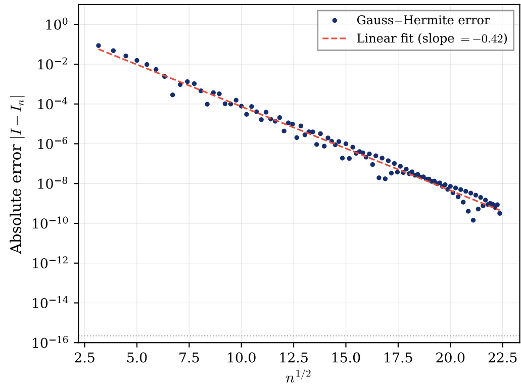
(a) Gauss–Hermite: O(e^{-C\sqrt{n}})
