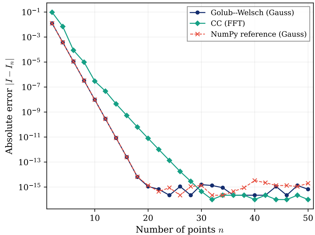
(b) f(x) = 1/(1 + x^2)
