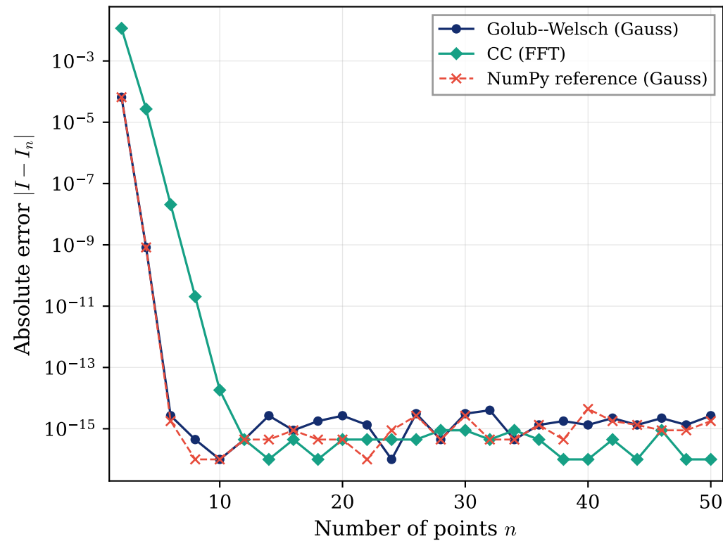
(a) f(x) = e^x
