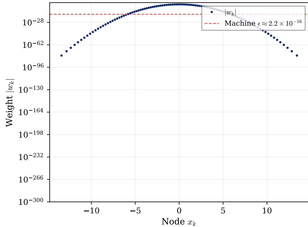
(a) Gauss–Hermite weights ( n = 100 )
