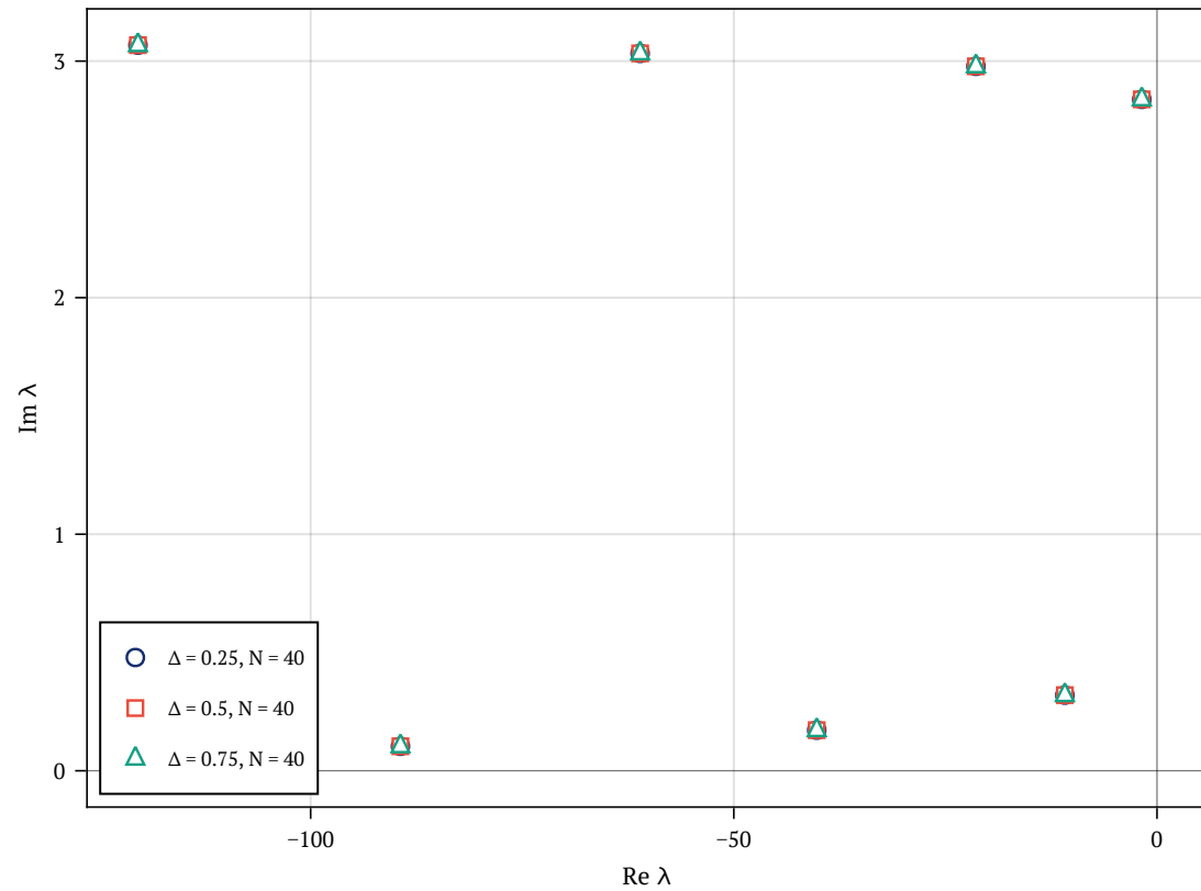
first eigenvalues in the complex plane
