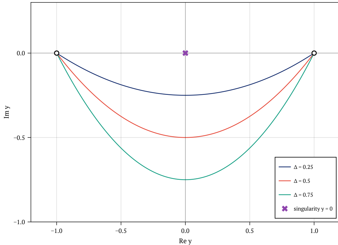
parabolic detour y(x) = x + i\Delta(x^2 - 1)
