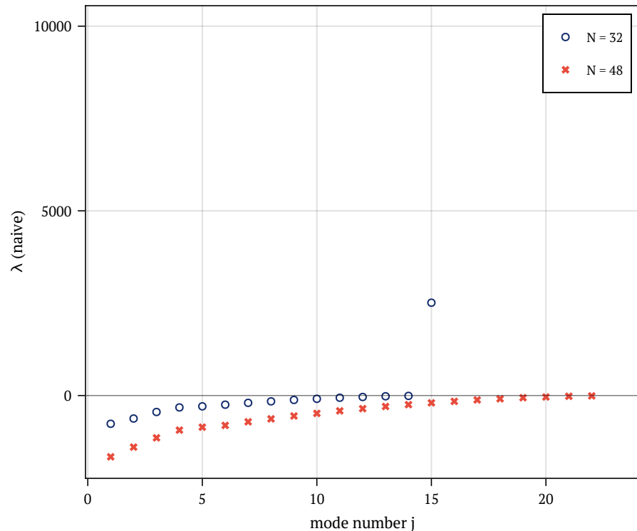
naive: 1 spurious \lambda > 0 at N=32, 1 at N=48
