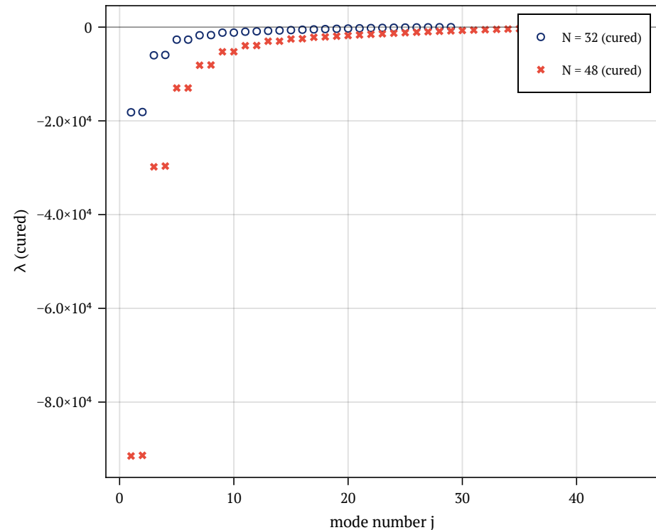
cured: 0 spurious at N=32, 0 at N=48
