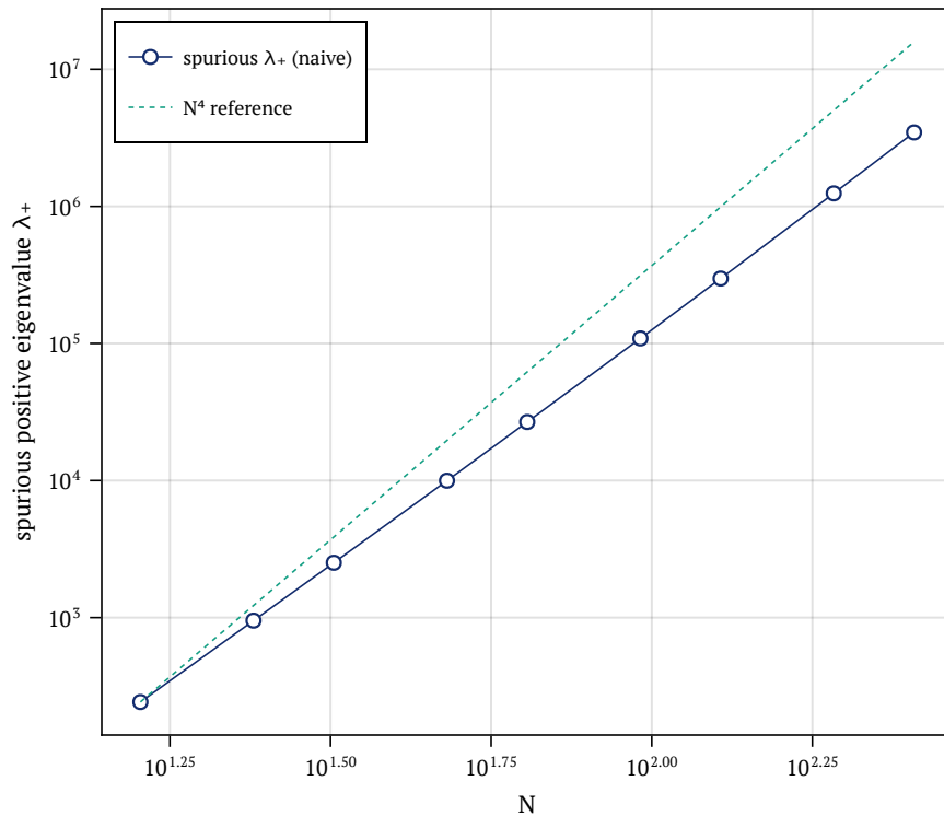
DDD scaling: empirical slope \approx 3.45 , asymptote N^4
