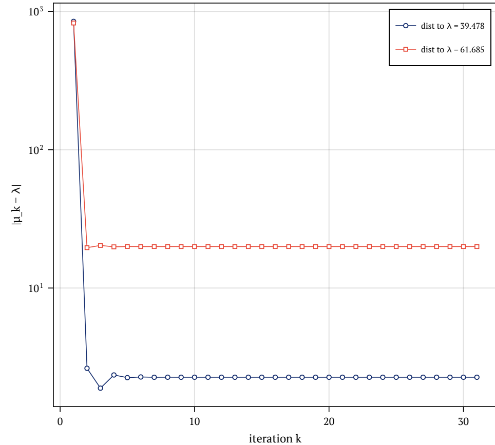
cautionary: \mu = 50.582 between two modes
