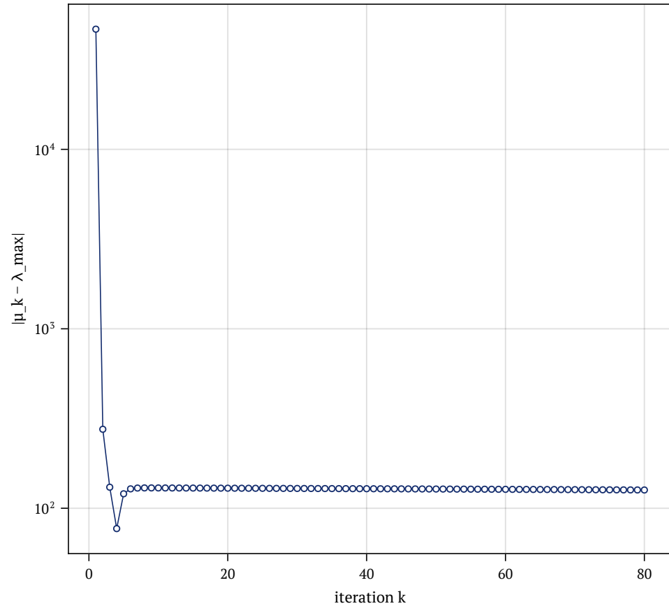
power method \rightarrow \lambda_{\max} = 49939.0 (stalls: |\lambda_{[N-1]} / \lambda_N| = 0.997 )
