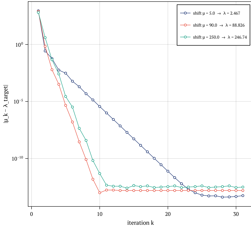
inverse iteration: three shifts, three modes
