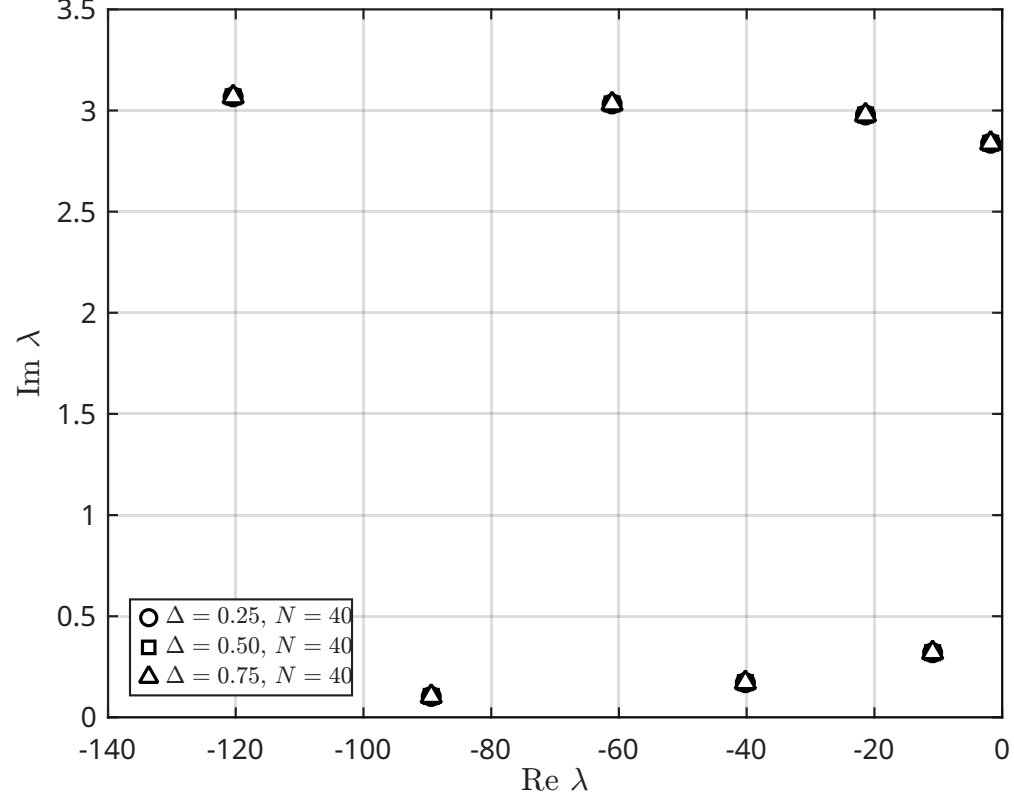
first eigenvalues in the complex plane
