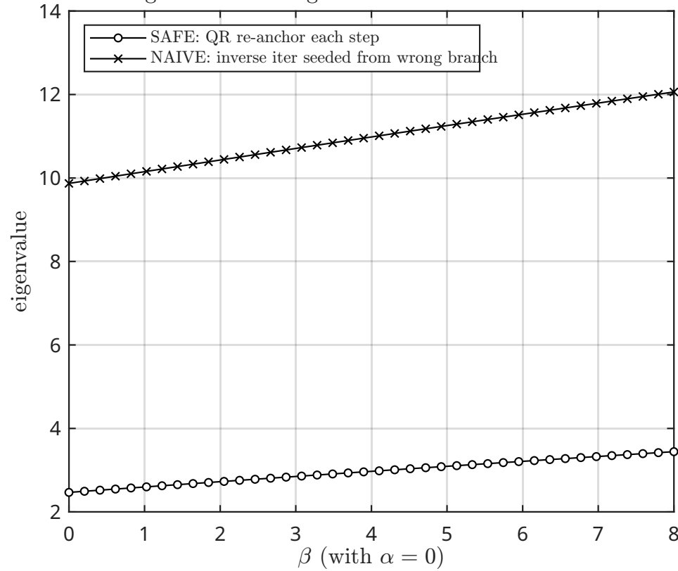
eigenvalue tracking: safe vs. naive local iteration
