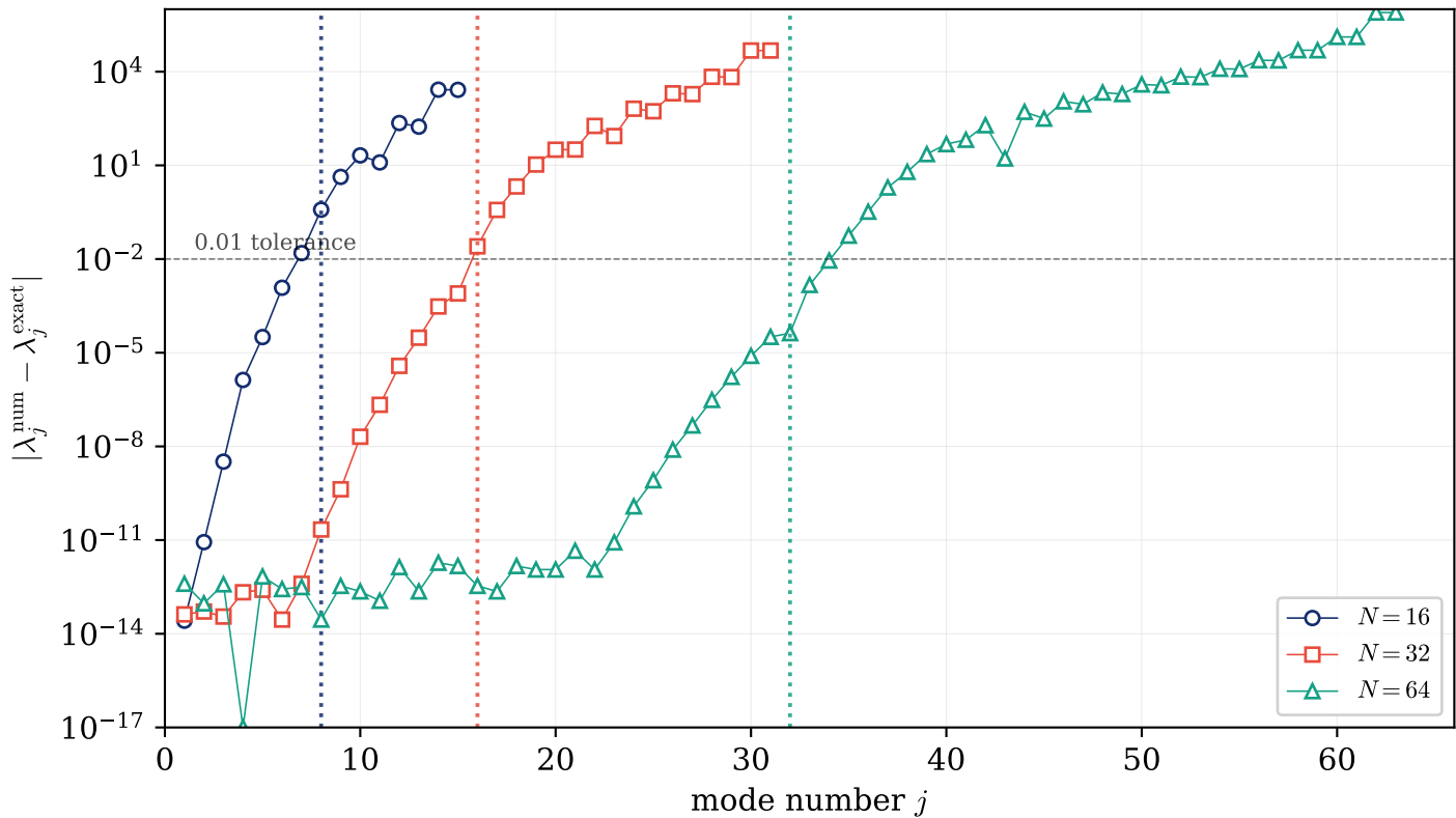
Dirichlet Laplacian: errors at three resolutions
