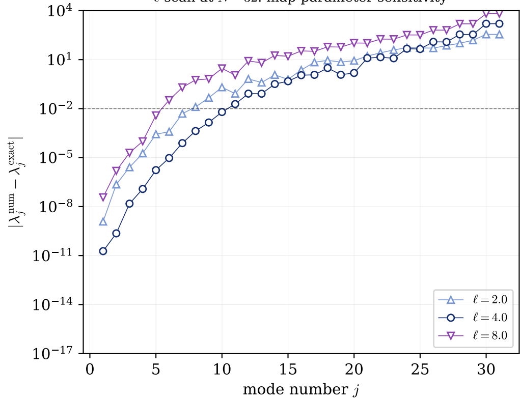
\ell -scan at N=32 : map-parameter sensitivity
