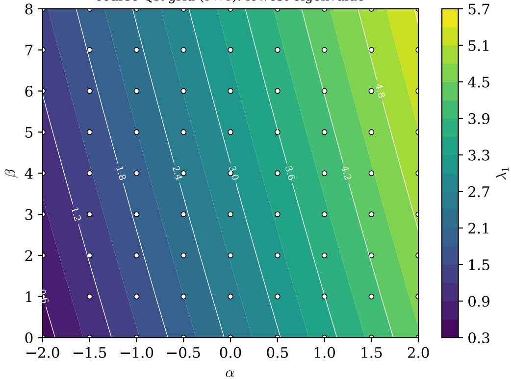
coarse QR grid ( 9 \times 9 ): lowest eigenvalue
