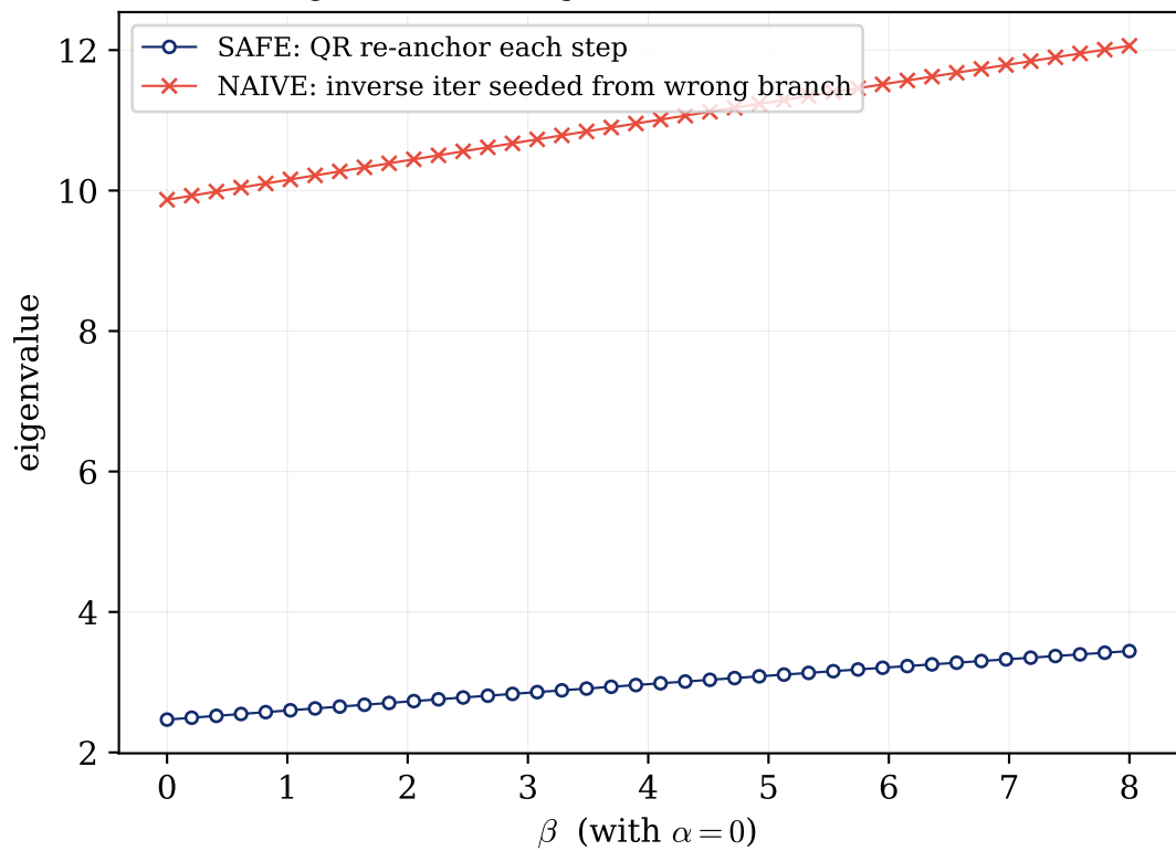
eigenvalue tracking: safe vs. naive local iteration
