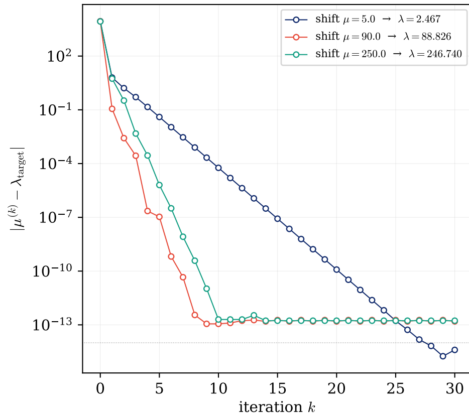
inverse iteration: three shifts, three modes
