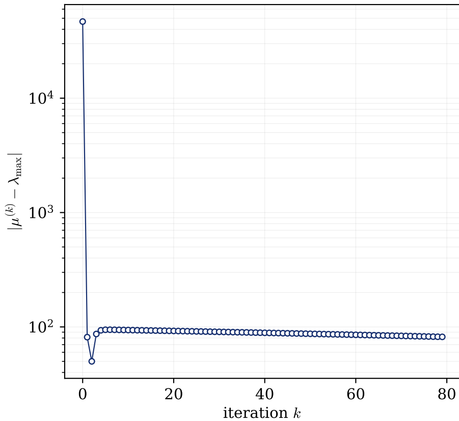
power method \rightarrow \lambda_{\max} = 49939 (stalls: |\lambda_{N-1}/\lambda_N| = 0.997 )
