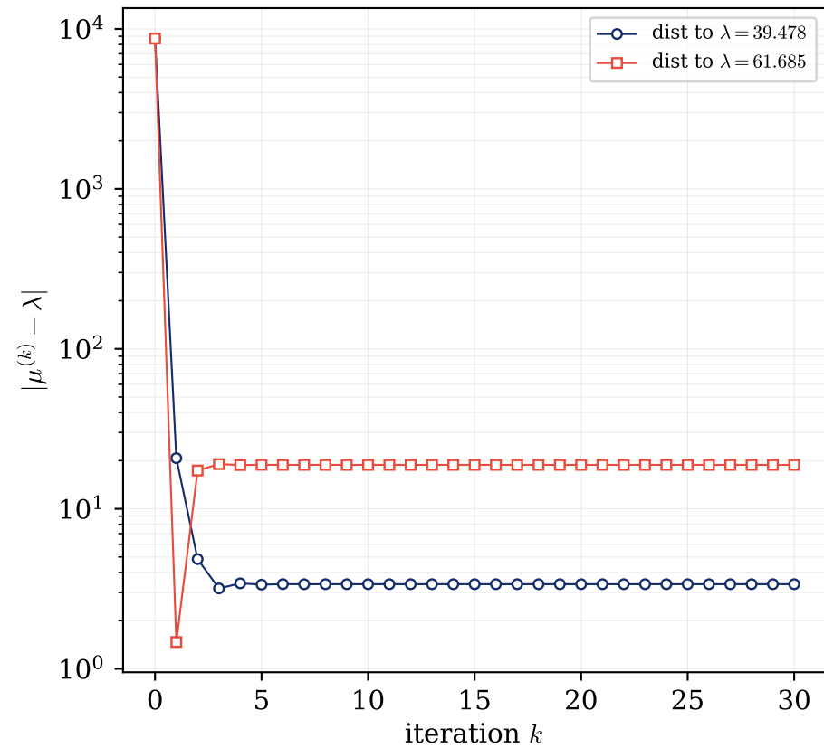
cautionary: shift \mu = 50.582 between two modes
