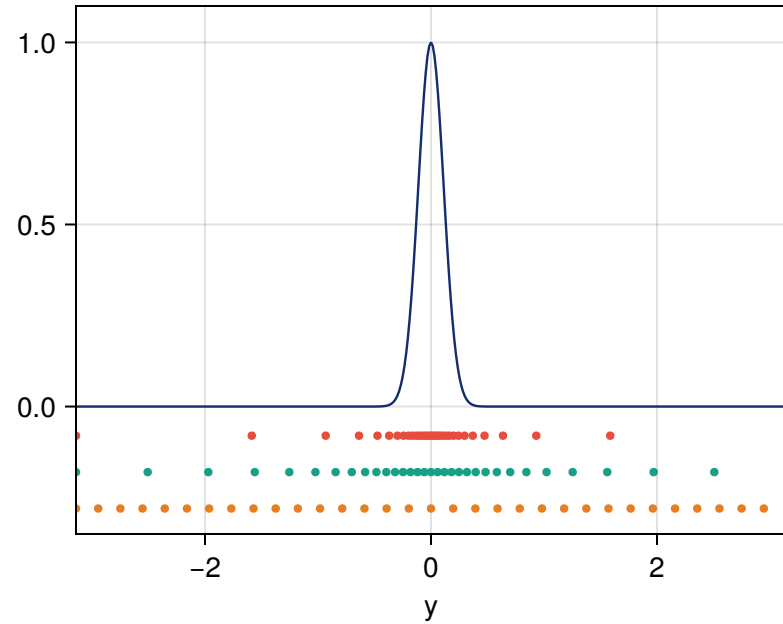
(a) Mapped grids, N=32
