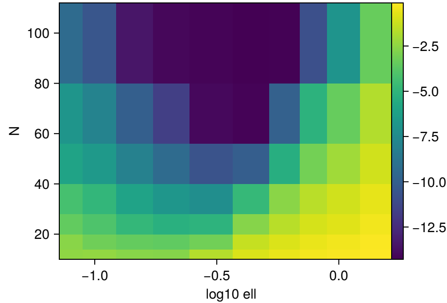
(b) Error landscape
