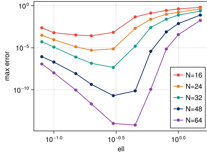
(c) Slices at fixed N
