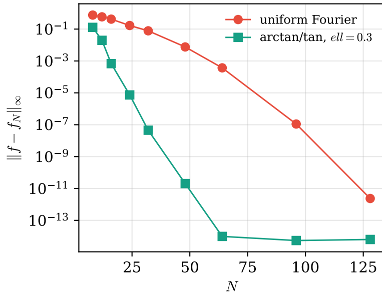
(b) Convergence
