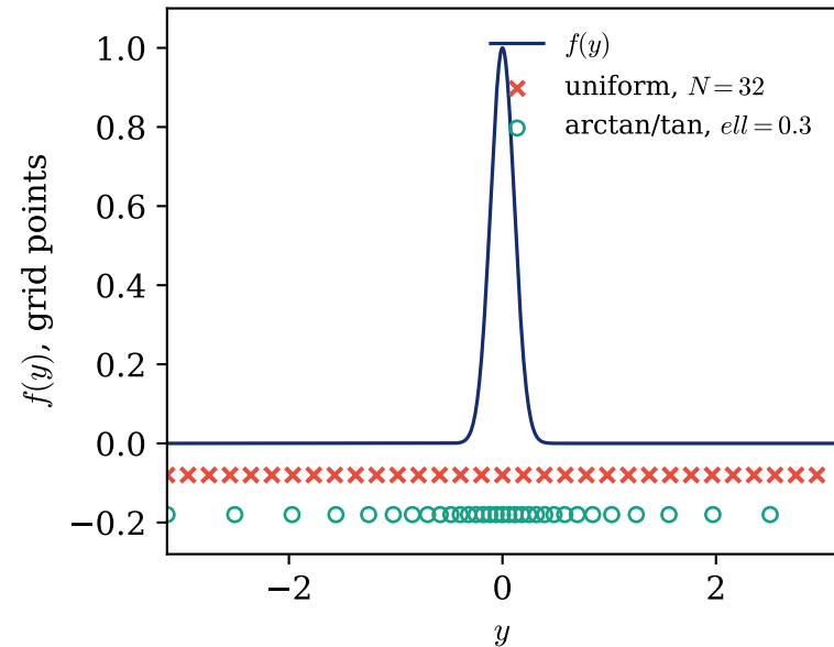
(a) Pulse + two grids
