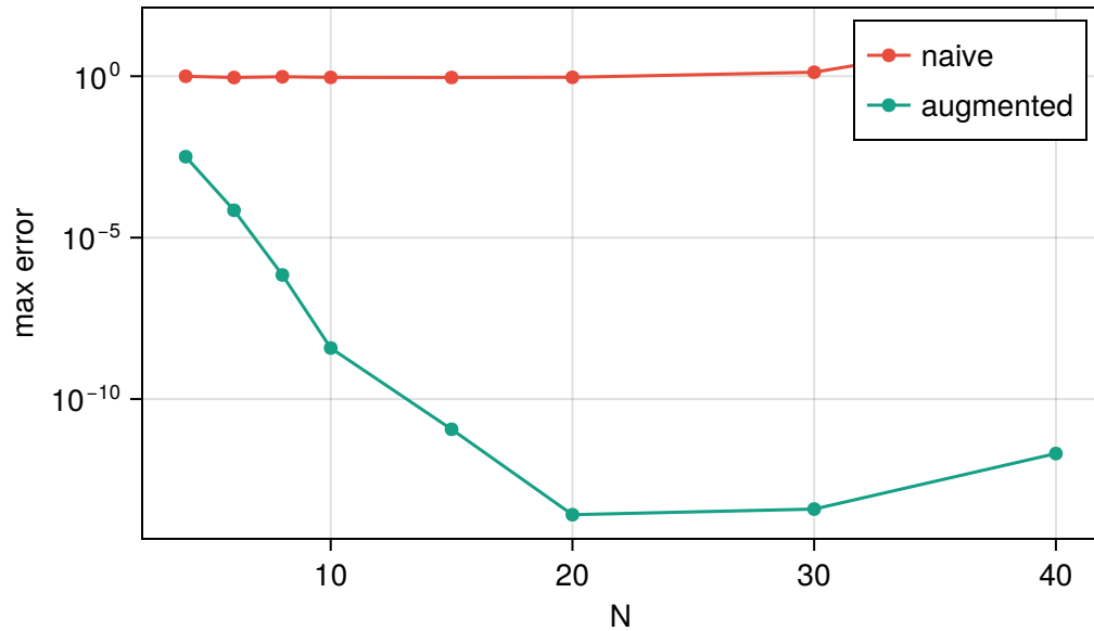
(b) Asymptotic augmentation wins
