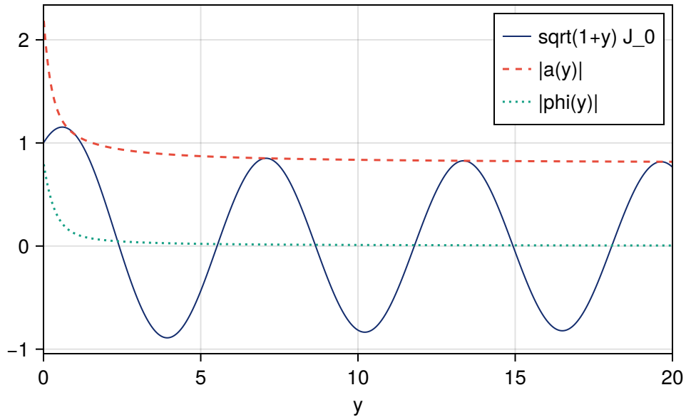
(a) \sqrt{1+y} J_0(y) with amp-phase decomposition
