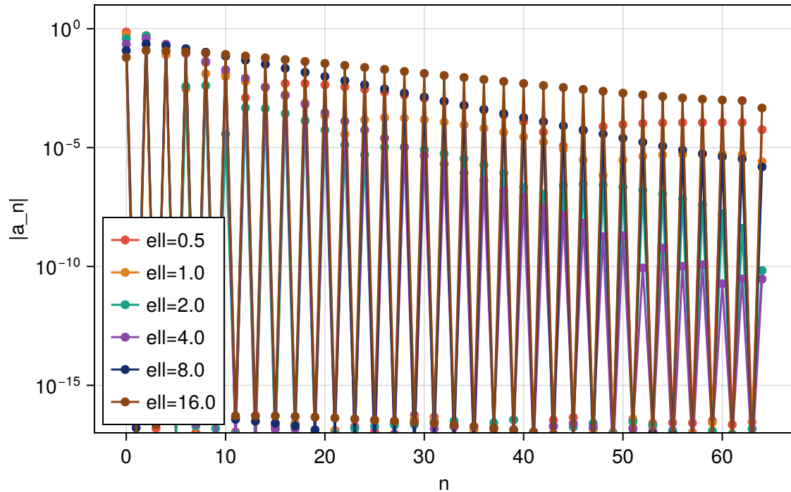
(a) Coefficient decay, N=64
