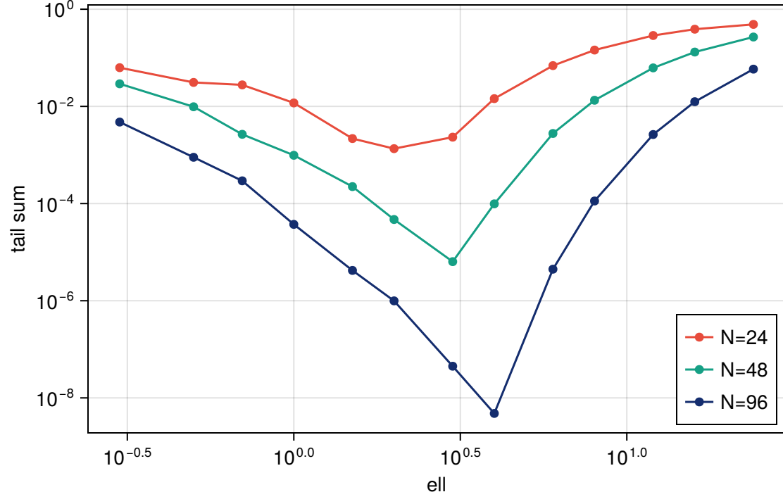
(b) Valley of good ell broadens with N
