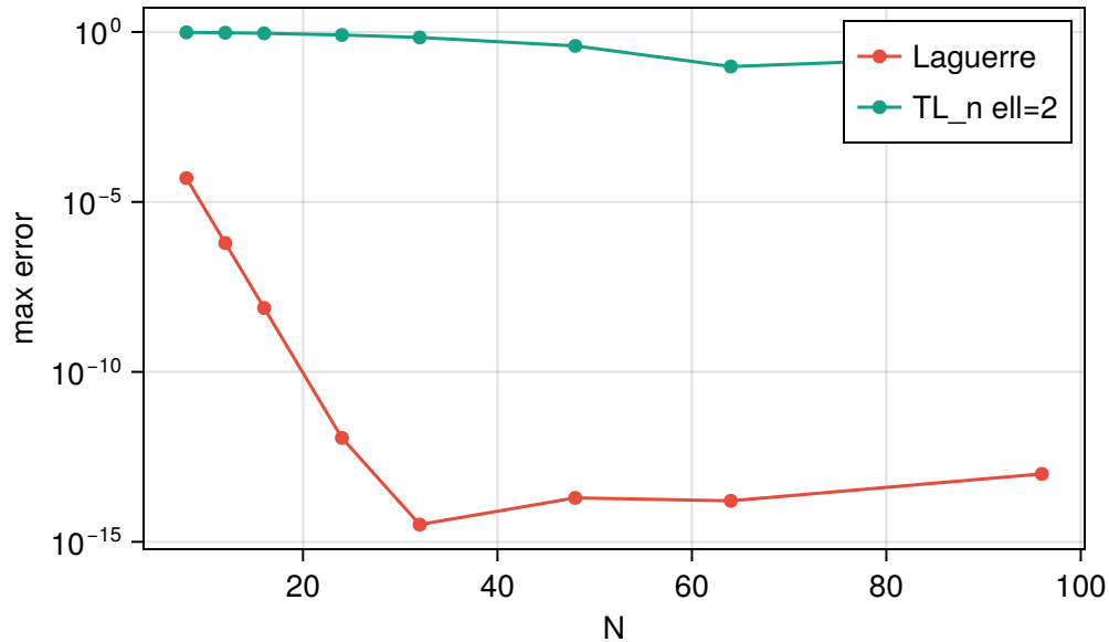
(a) f = e^{-y} (exponential)
