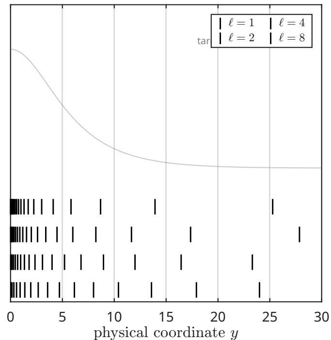
(b) collocation grids at N = 24 for several \ell
