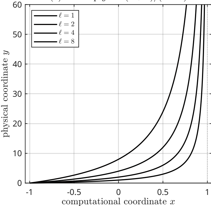
(a) the map y = \ell(1+x)/(1-x)
