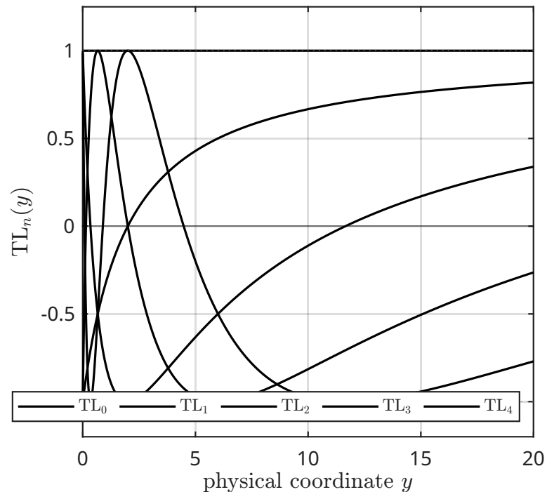
(c) basis functions \text{TL}_0, \dots, \text{TL}_4 at \ell = 2
