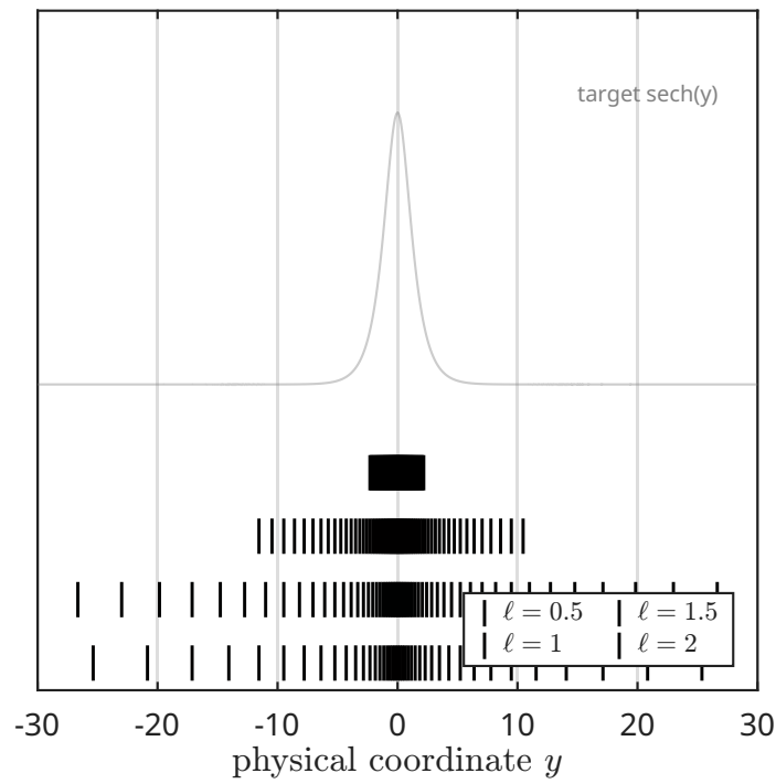
(b) sinh-mapped grids at N = 64 for several \ell
