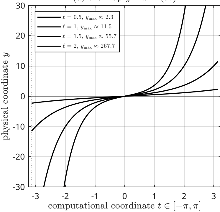
(a) the map y = \sinh(\ell t)
