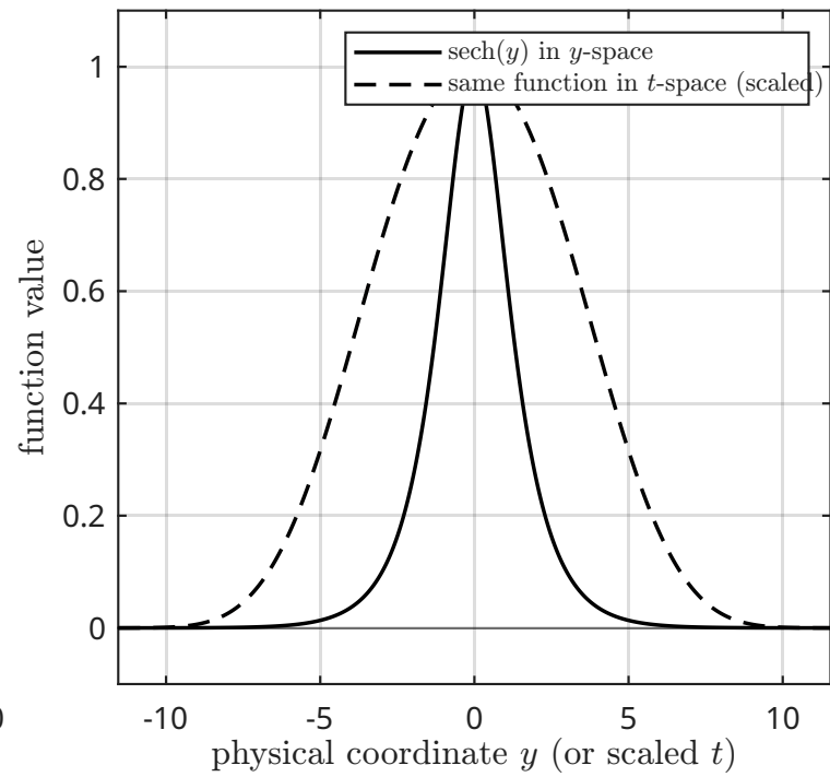
(c) \text{sech}(y) in two coordinate frames at \ell = 1
