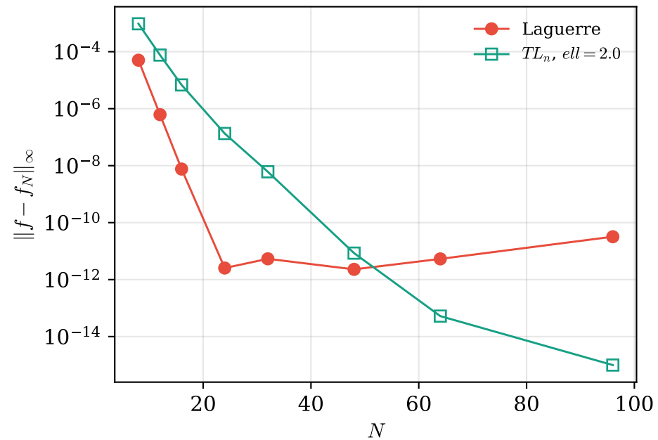
(a) f(y) = e^{-y} (exponential decay)
