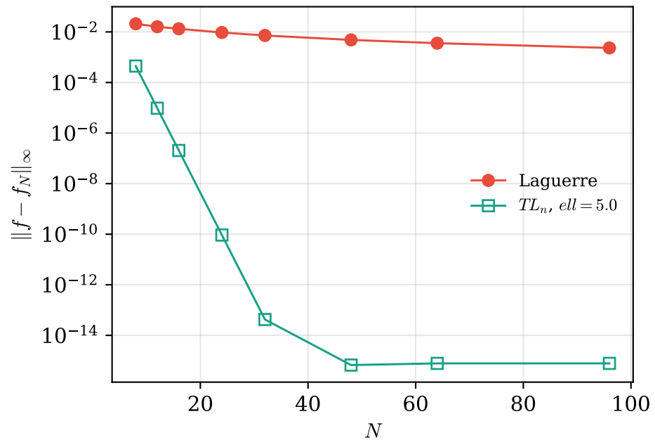
(b) f(y) = 1/(1 + y) (algebraic decay)
