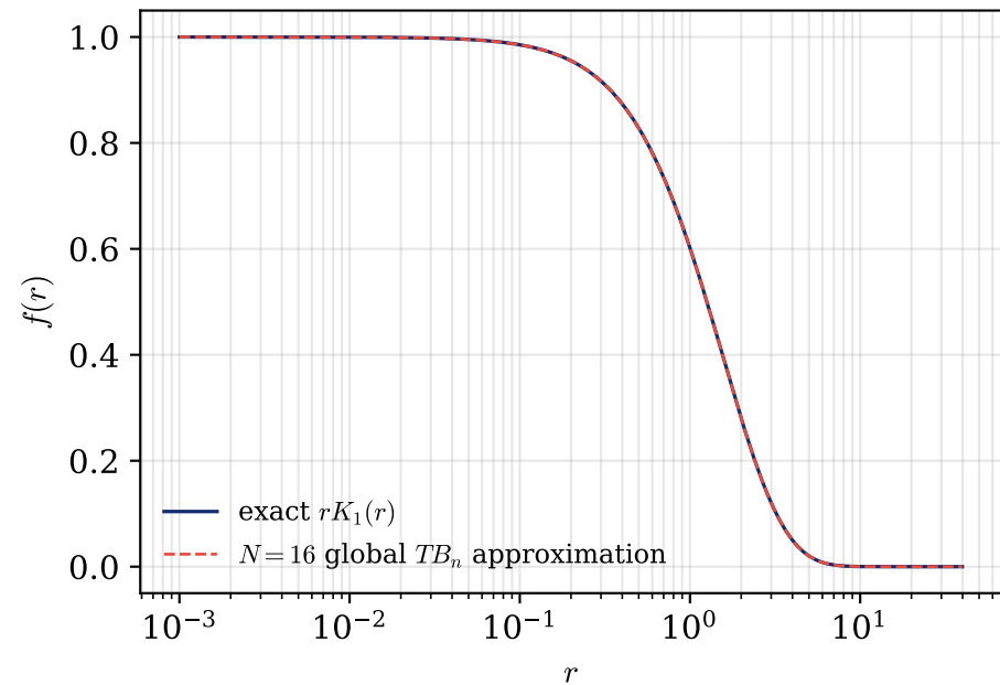
(a) Global expansion of rK_1(r)
