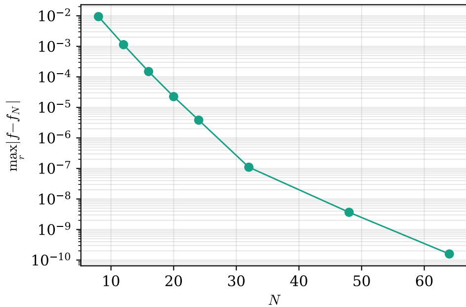
(b) Subgeometric descent, ell = 4.0
