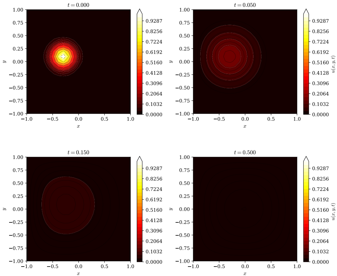
Figure 60: Solution of the 2D heat equation Equation 133. Four snapshots at times t = 0 , 0.05, 0.15, and 0.5. The initial hot spot diffuses isotropically, spreading and decaying towards the zero steady state.
