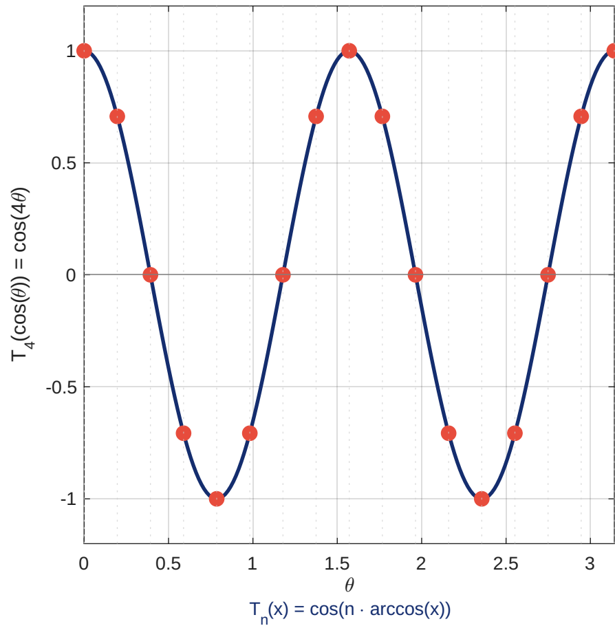
Chebyshev Polynomial T_4 as Cosine Wave
