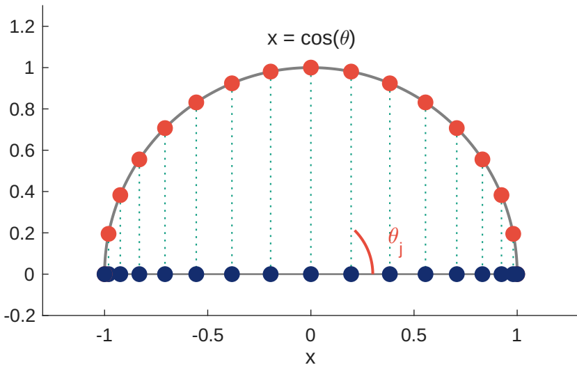
Chebyshev Points from Circle Projection
