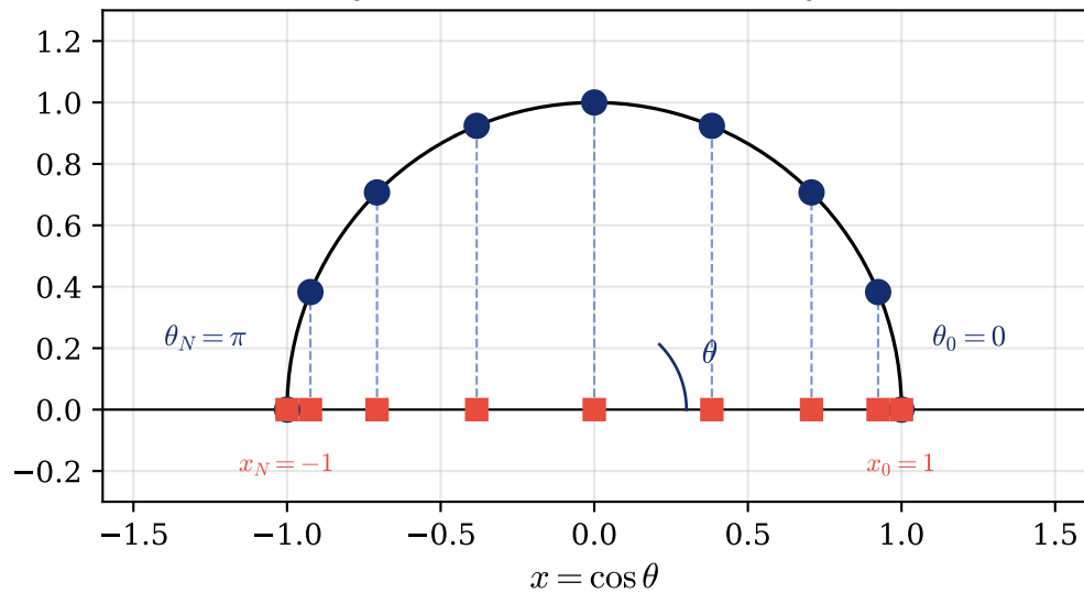
Chebyshev points as circle projection
