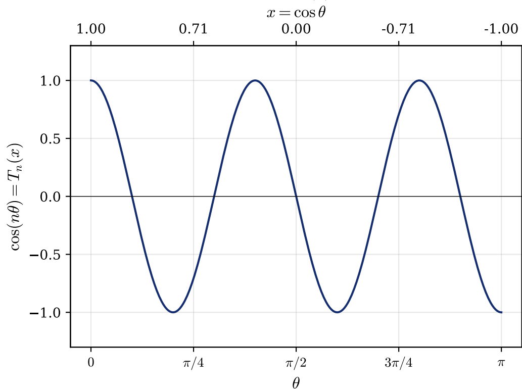
Chebyshev polynomial T_5(x) as wrapped cosine
