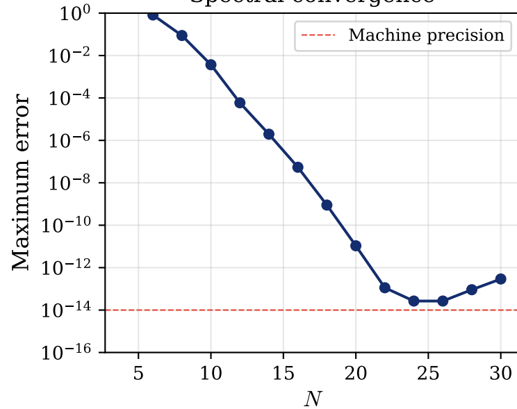
Spectral convergence
