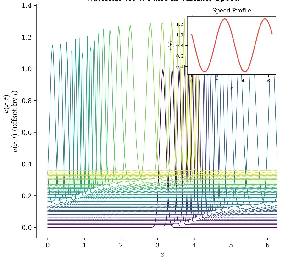
Waterfall View: Pulse in Variable Speed
