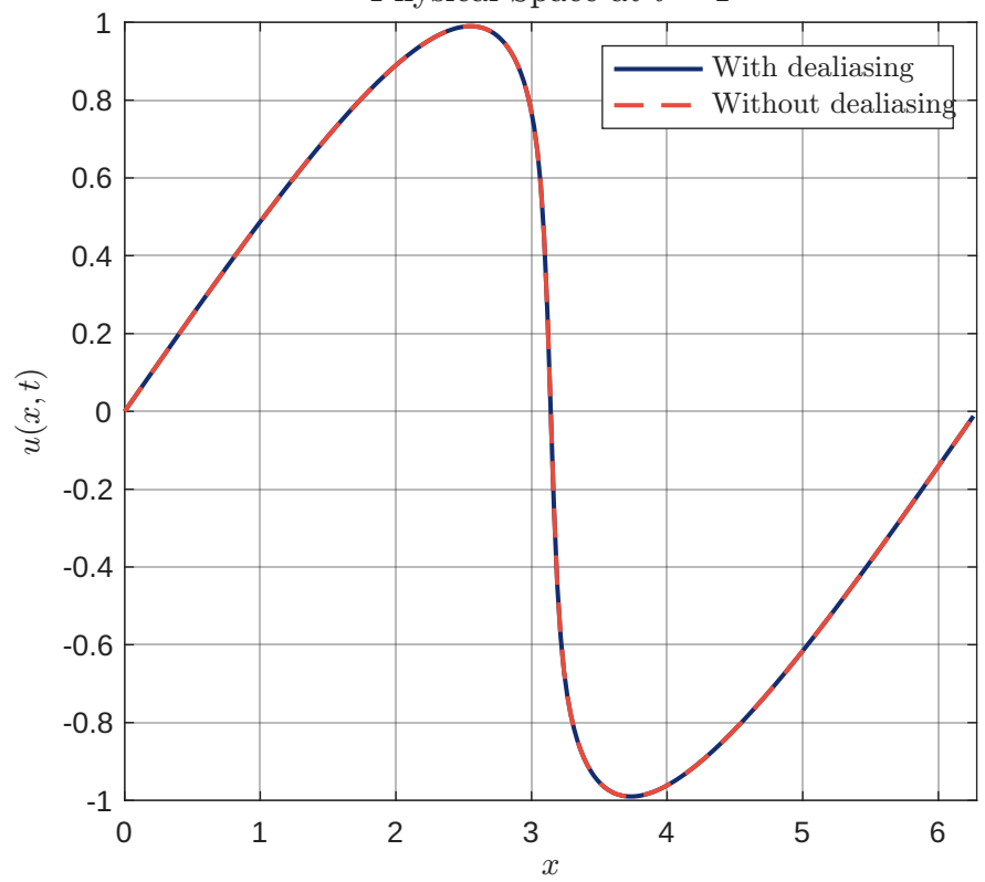
Physical Space at t = 1
