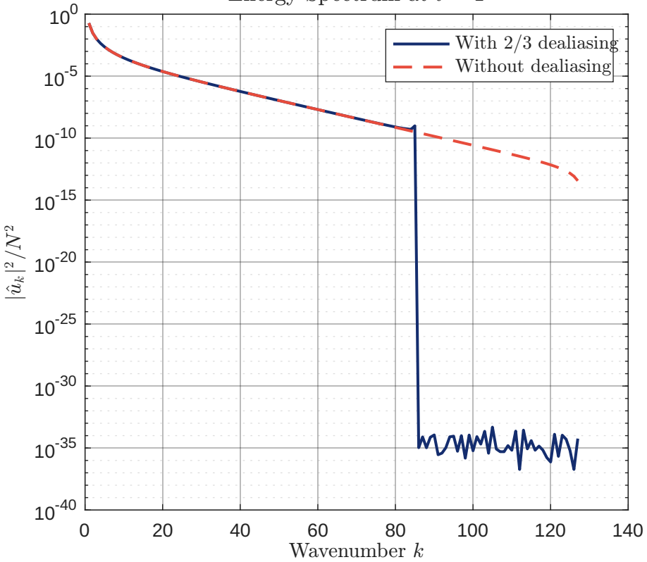
Energy Spectrum at t = 1
