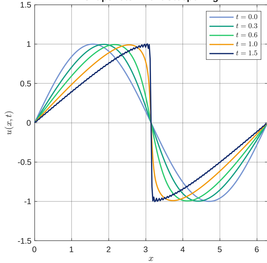
Snapshots: Front Steepening
