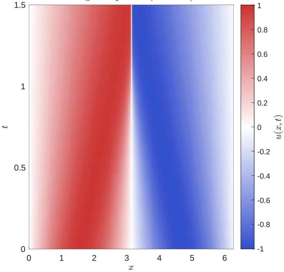
Burgers Equation ( \nu = 0.01 )
