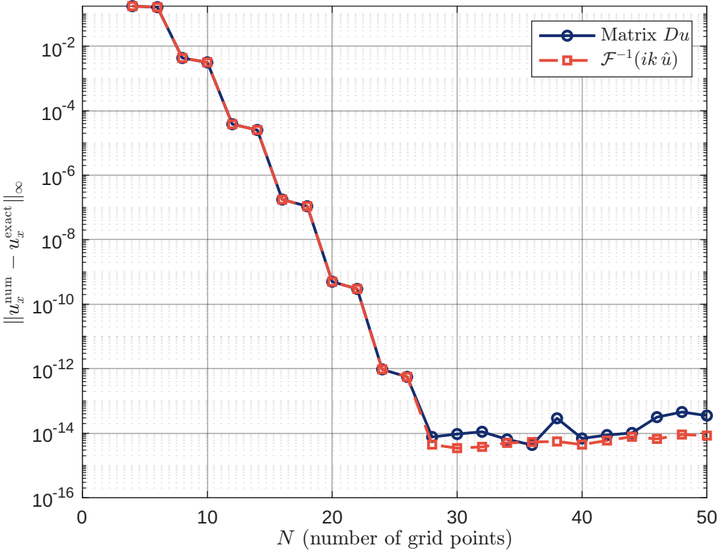
Spectral Convergence: u(x) = e^{\sin x}
