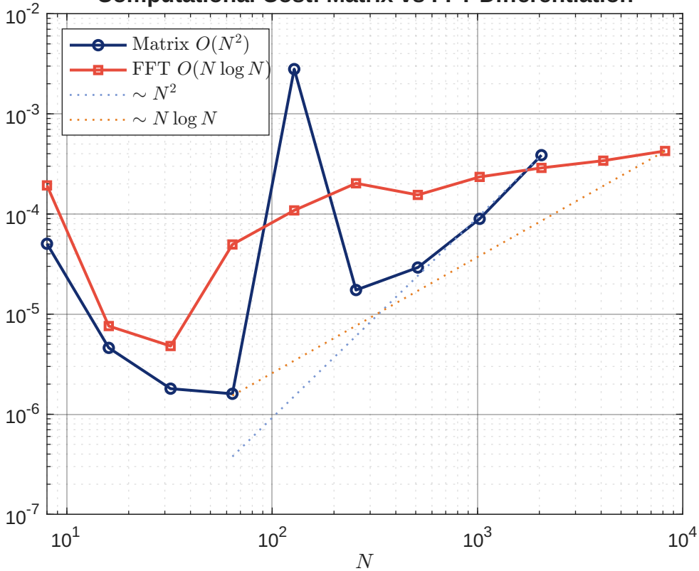
Computational Cost: Matrix vs FFT Differentiation
