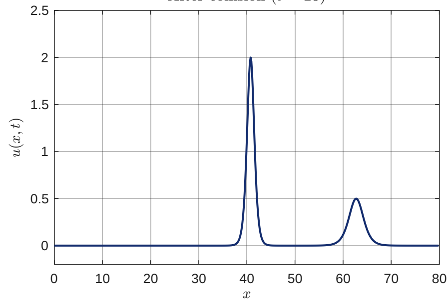
After collision ( t = 25 )
