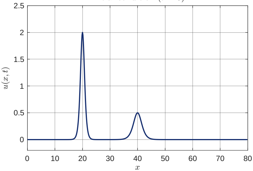
Initial condition ( t = 0 )
