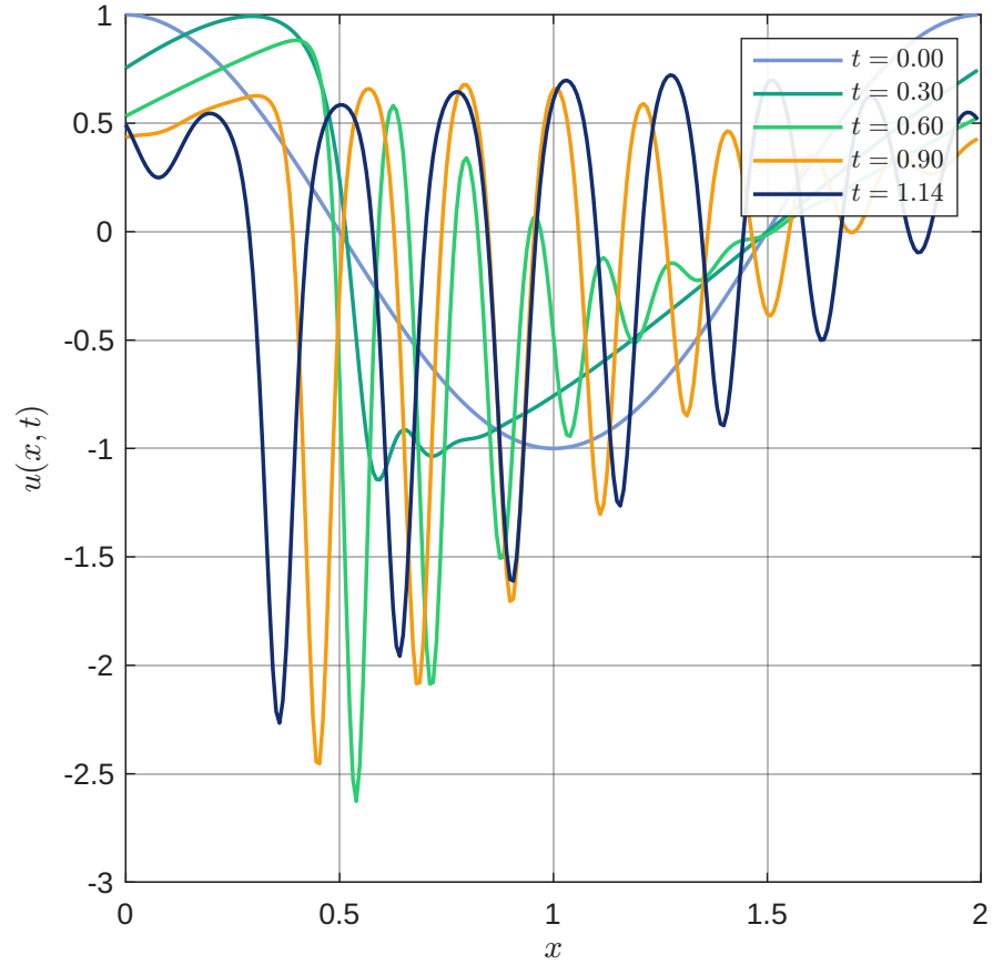
Soliton Train Formation
