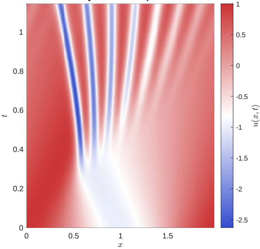
Zabusky--Kruskal Experiment
