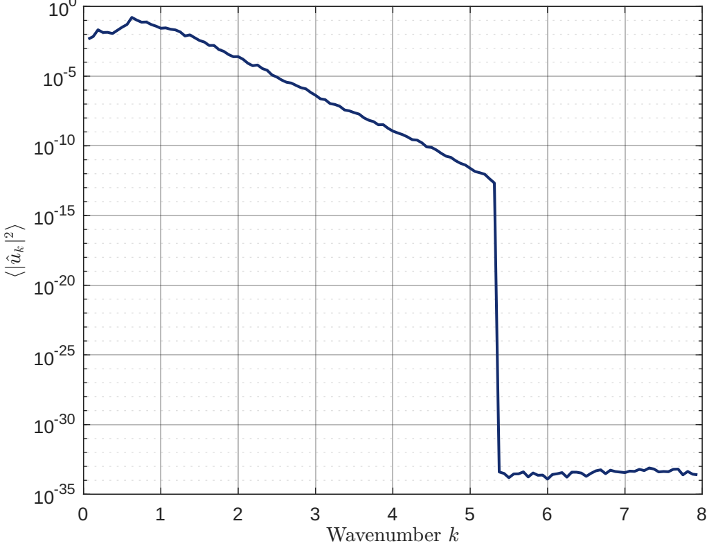
Time-Averaged Energy Spectrum (KS)
