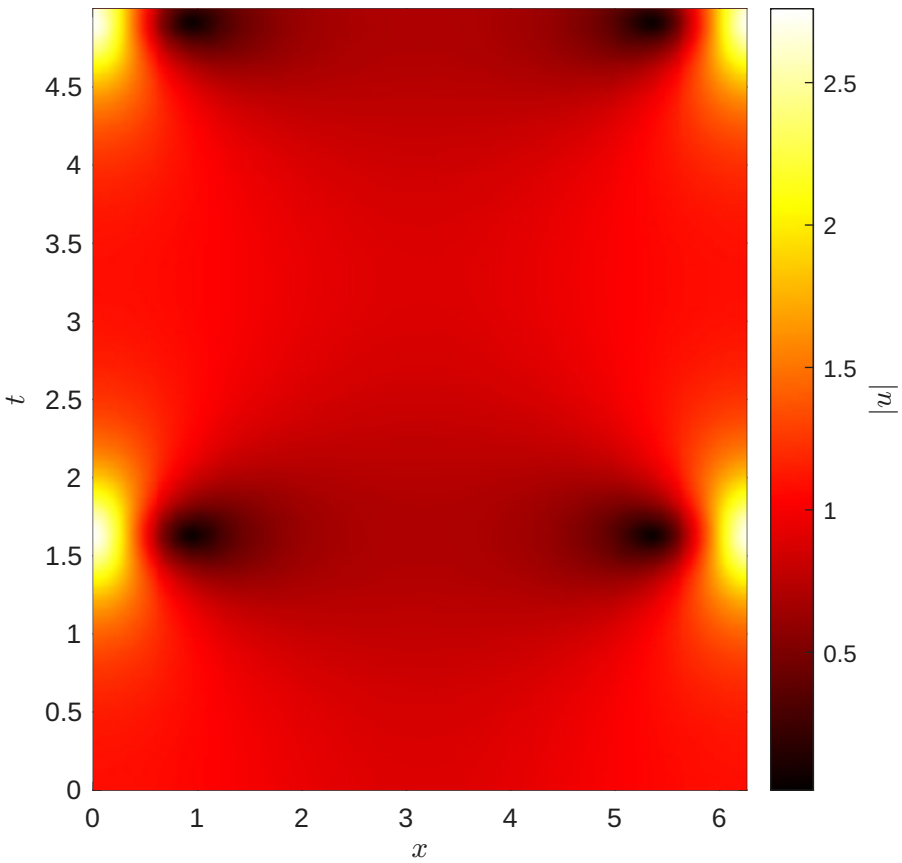
NLS: |u(x, t)| (Modulation Instability)
