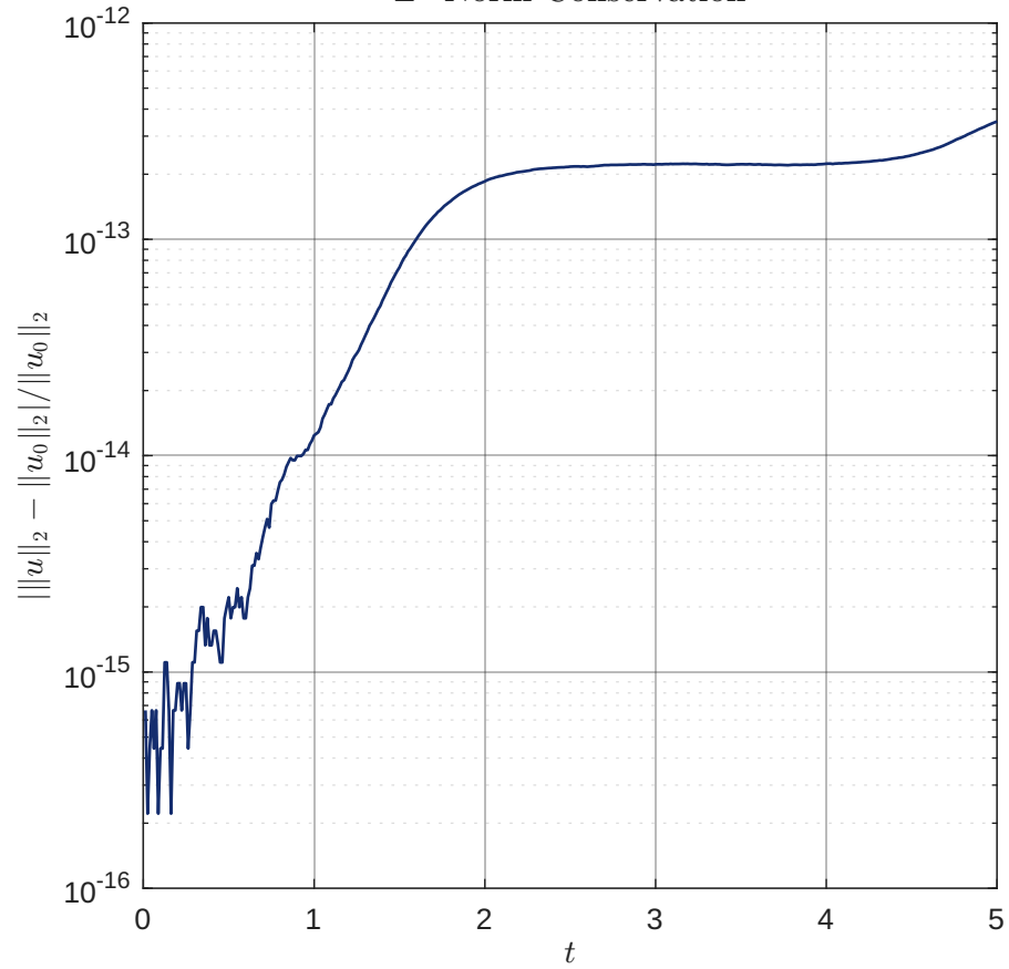
L^2 Norm Conservation
