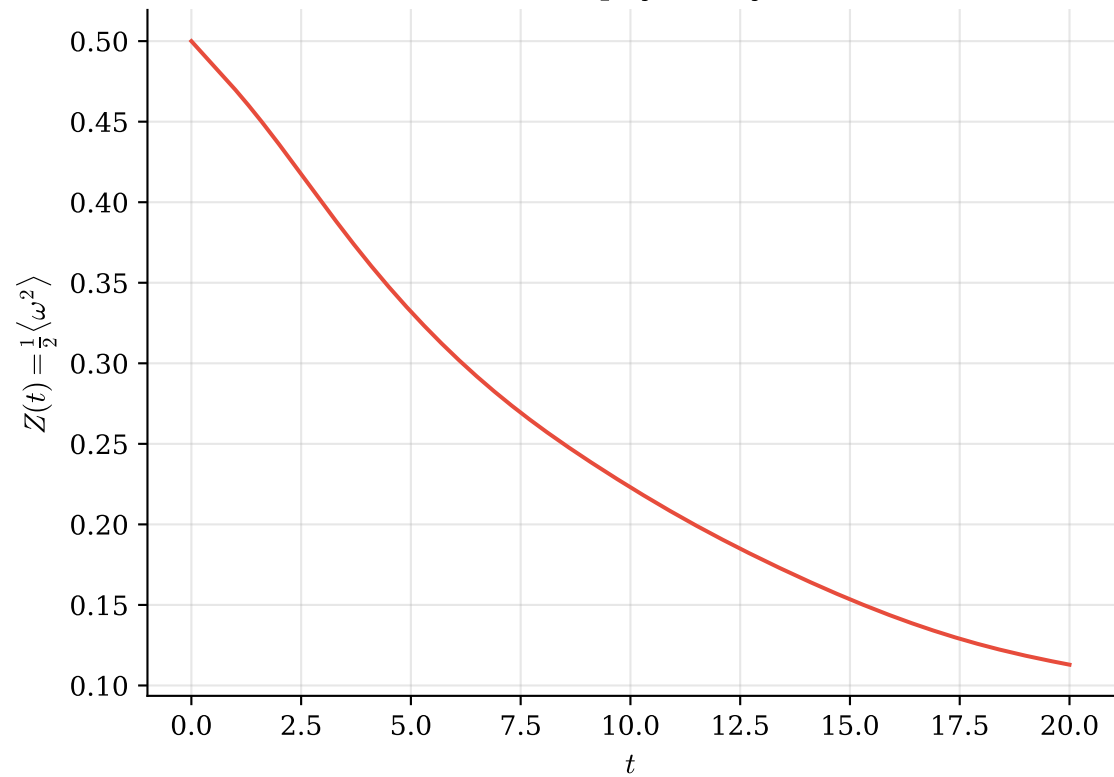
Enstrophy Decay
