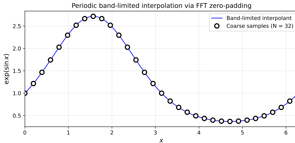
Figure 54: Band-limited interpolation via zero-padding. Black dots show N = 32 samples of \exp(\sin x) . The solid curve shows the interpolant obtained by zero-padding the FFT to M = 128 points. The interpolant passes exactly through the original samples and provides a smooth reconstruction between them.
