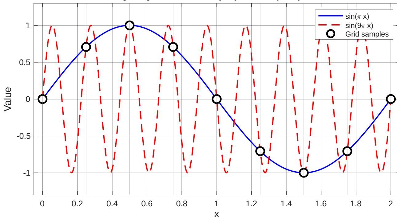
Aliasing on grid h = 1/4 : \sin(\pi x) and \sin(9\pi x) coincide
