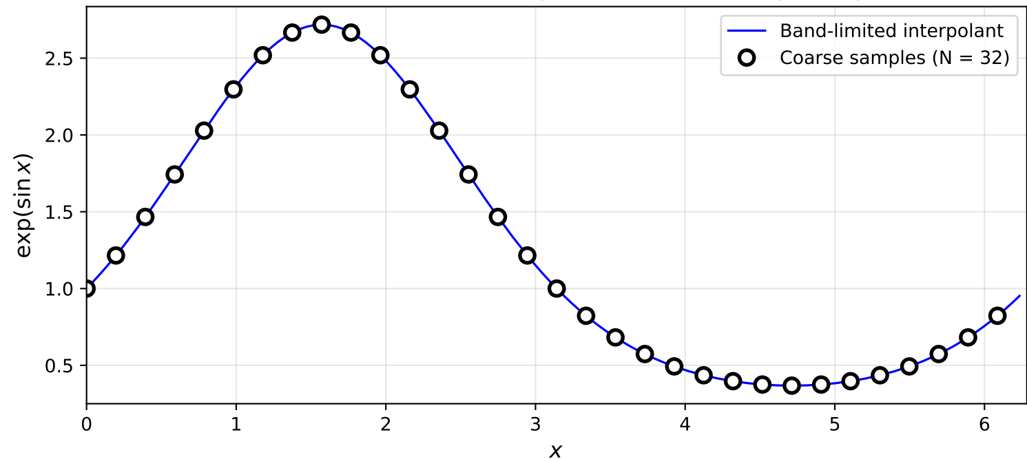
Periodic band-limited interpolation via FFT zero-padding
