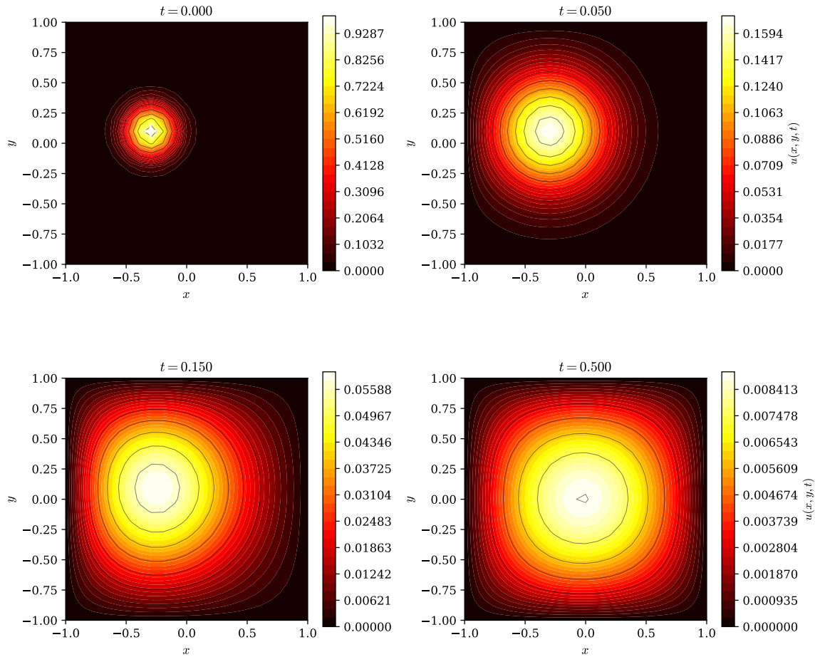
Figure 63: Solution of the 2D heat equation Equation 149. Four snapshots at times t = 0, 0.05, 0.15 , and 0.5 . The initial hot spot diffuses isotropically, spreading and decaying towards the zero steady state.
