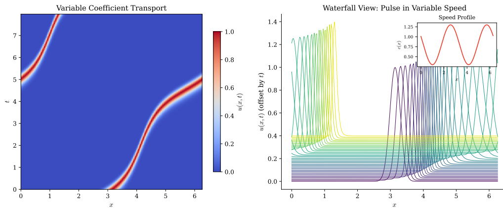
Figure 65: Solution of the variable-coefficient transport equation Equation 159. Left: space-time diagram showing the characteristic trajectory of a Gaussian pulse in a medium where c(x) = 0.3 + \sin^2(x - 1) . The pulse accelerates in fast regions and decelerates in slow regions. Right: waterfall view of the same solution with vertical offset proportional to time.
