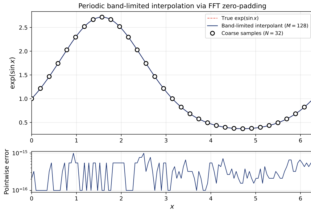
Figure 57: Band-limited interpolation via zero-padding. Top: the true function \exp(\sin x) (dashed), the interpolant from zero-padding to M = 128 points (solid), and the N = 32 coarse samples (circles). The curves are visually indistinguishable. Bottom: pointwise error |p(x) - f(x)| on a logarithmic scale, confirming machine-precision accuracy for this analytic function.
