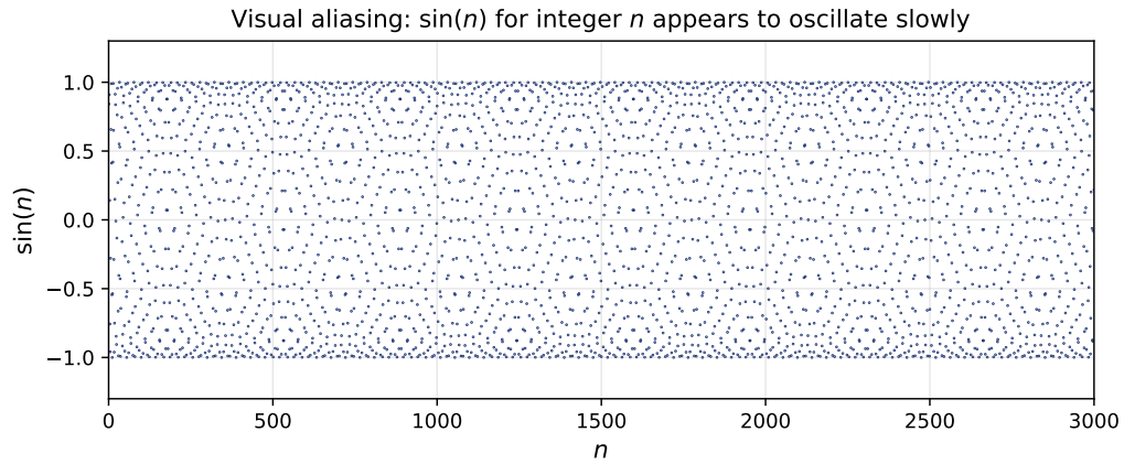
Figure 55: Visual aliasing: \sin(n) for integer n = 1, \dots, 3000 . Although the function oscillates rapidly (nearly one radian per step), the plotted points appear to trace a slowly varying envelope. The eye, acting as a sampler, aliases the high frequency to a low-frequency pattern.
