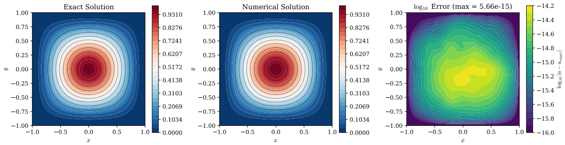
Figure 64: Solution of the 2D Poisson equation Equation 153 with manufactured solution Equation 154. Left: Exact solution. Centre: Numerical solution (visually indistinguishable from exact). Right: Error on a logarithmic scale, showing machine-precision accuracy throughout the interior. The spectral method achieves essentially exact results for this smooth problem.
