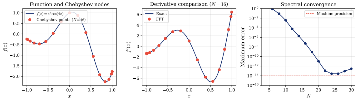
Figure 59: Chebyshev differentiation via FFT applied to f(x) = e^x \cos(4x) . Left: The function f(x) on [-1, 1] with Chebyshev nodes marked. Centre: Comparison of exact and FFT-computed derivative for N = 16 . Right: Maximum error versus N on a semilog scale, showing the characteristic straight-line descent of spectral convergence until machine precision is reached around N = 24 .
