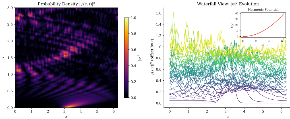
Figure 66: Solution of the Schrödinger equation Equation 161 with harmonic potential using Strang splitting. Left: space-time evolution of the probability density |u(x,t)|^2 showing the oscillatory dynamics of a Gaussian wavepacket in the harmonic trap. Right: waterfall plot of |u(x,t)|^2 at selected times.
