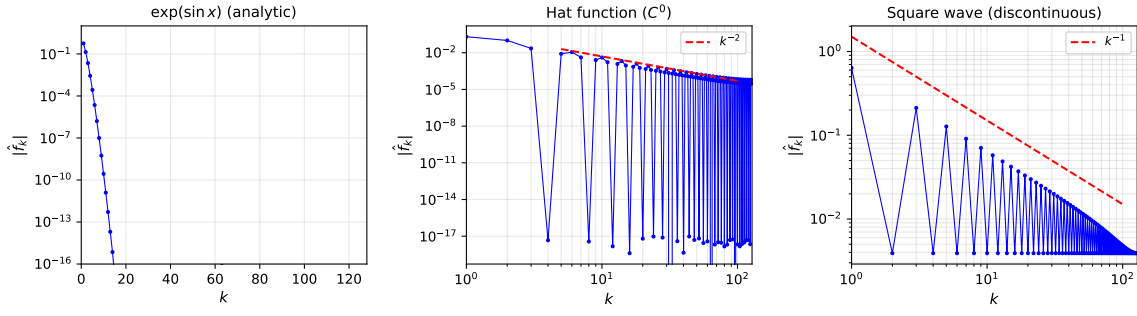
Figure 56: Fourier spectra of three functions with different smoothness. Left: \exp(\sin x) (analytic) shows exponential decay on a semilog plot. Center: Periodic hat function ( C^0 ) shows algebraic decay \approx |k|^{-2} on a log-log plot. Right: Square wave (discontinuous) shows slow decay \approx |k|^{-1} .
