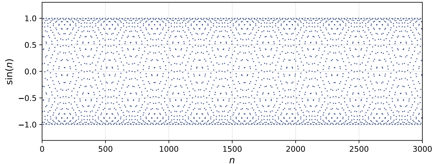
Visual aliasing: \sin(n) for integer n appears to oscillate slowly
