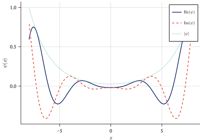
Fundamental mode (n = 0): \omega = 1.3227 - 0.5002i
