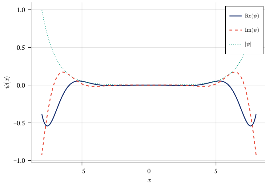
A spurious mode: \omega = 1.3424 - 0.9723i
