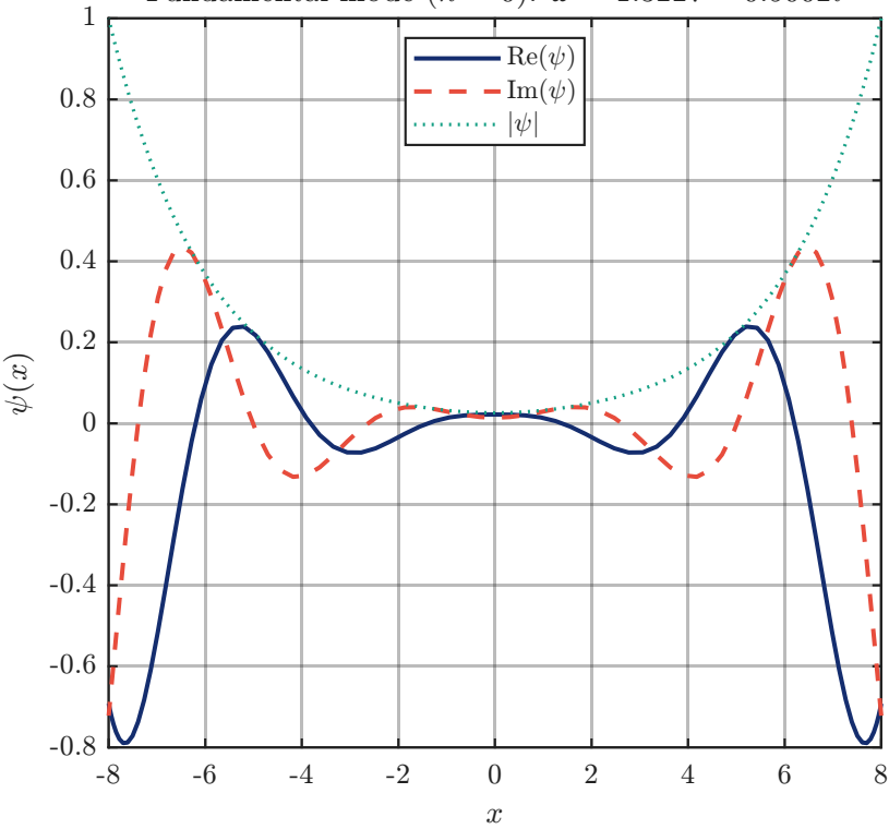
Fundamental mode ( n = 0 ): \omega = 1.3227 - 0.5002i
