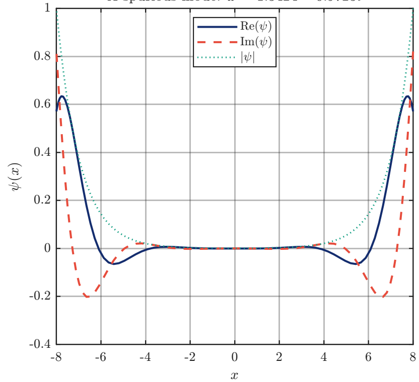
A spurious mode: \omega = 1.3424 - 0.9723i
