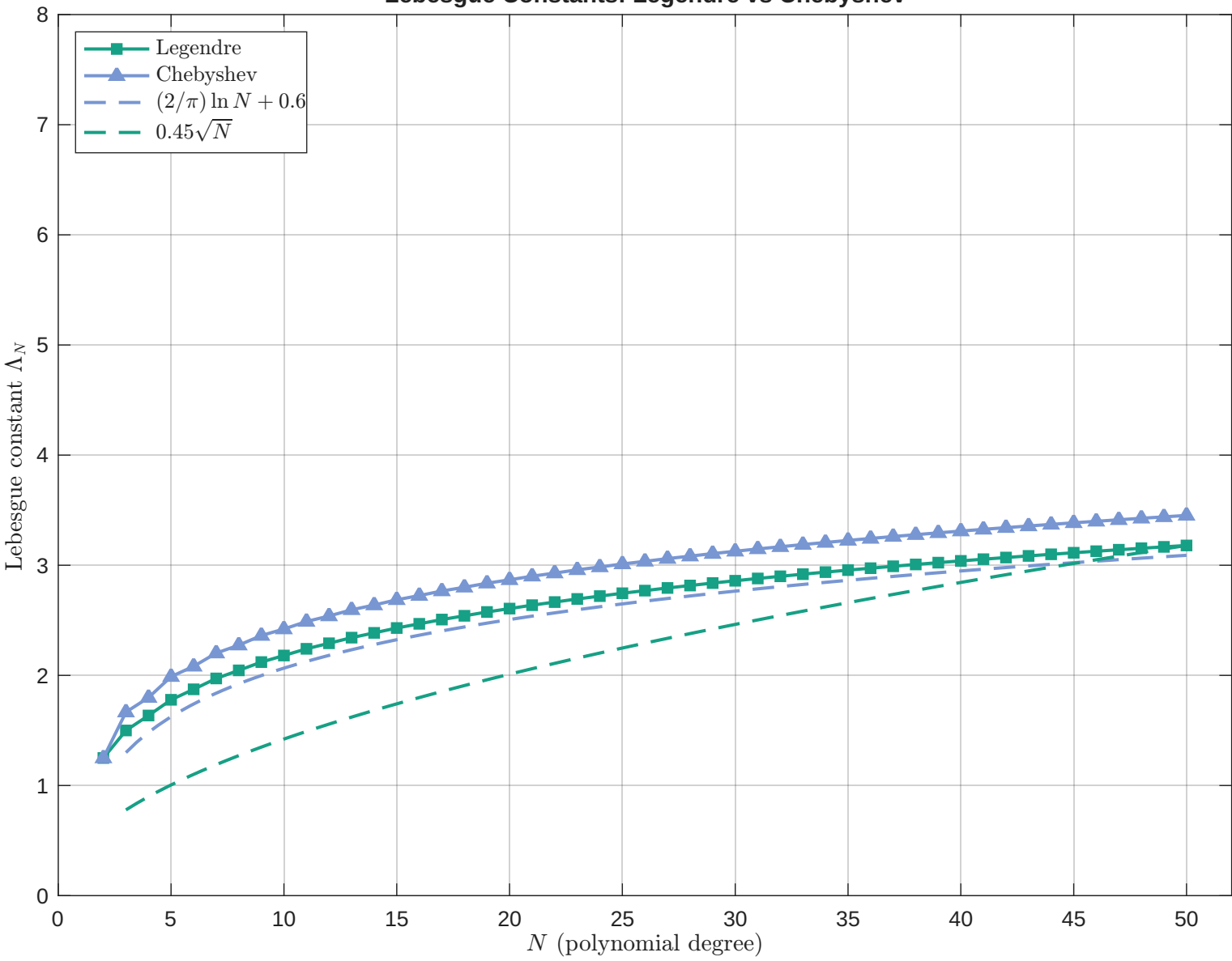
Lebesgue Constants: Legendre vs Chebyshev
