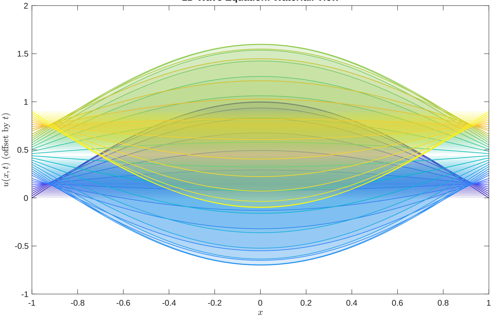
1D Wave Equation: Waterfall View
