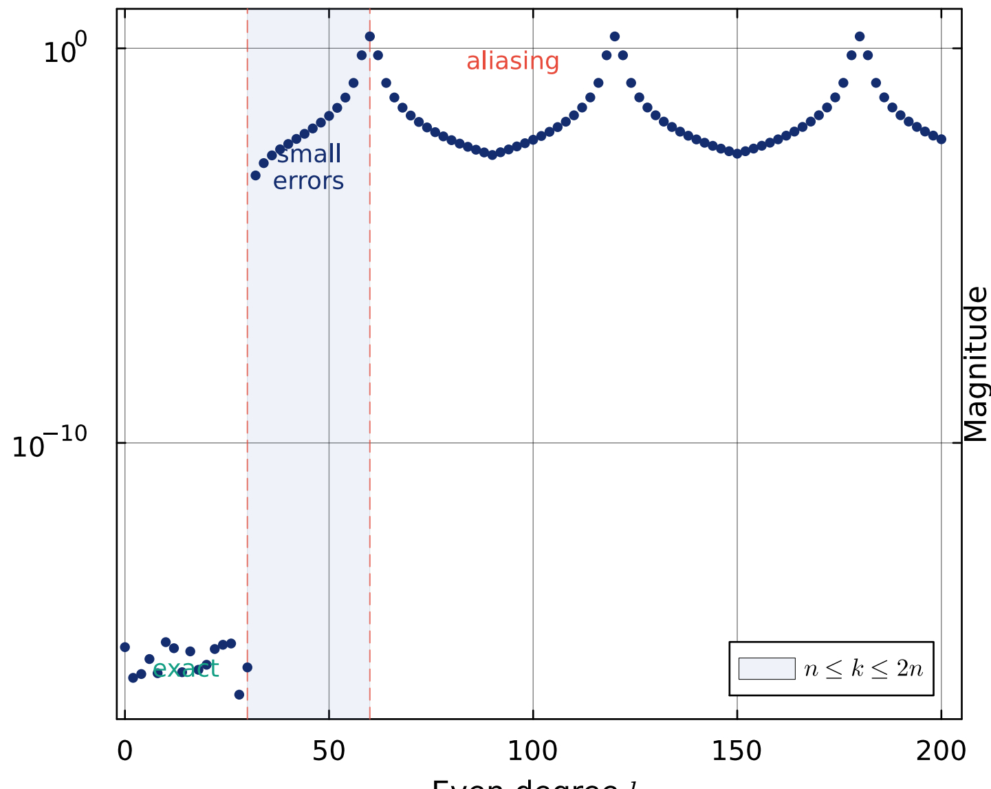
(a) CC error for Chebyshev polynomials ( n = 30 )
