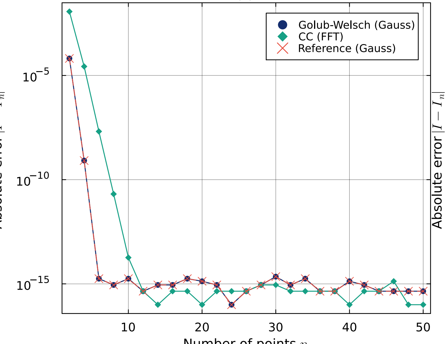
(a) f(x) = e^x
