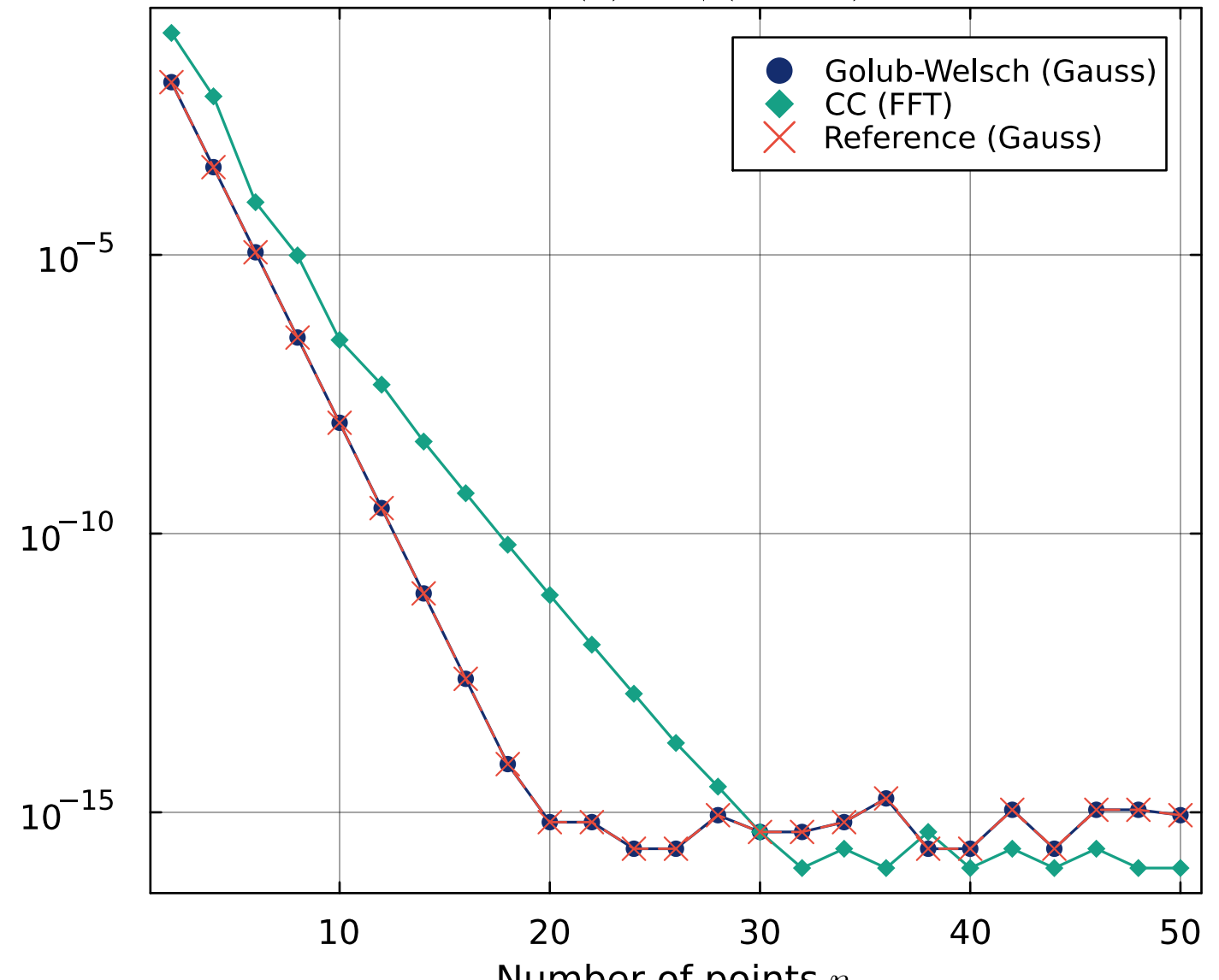
(b) f(x) = 1/(1 + x^2)
