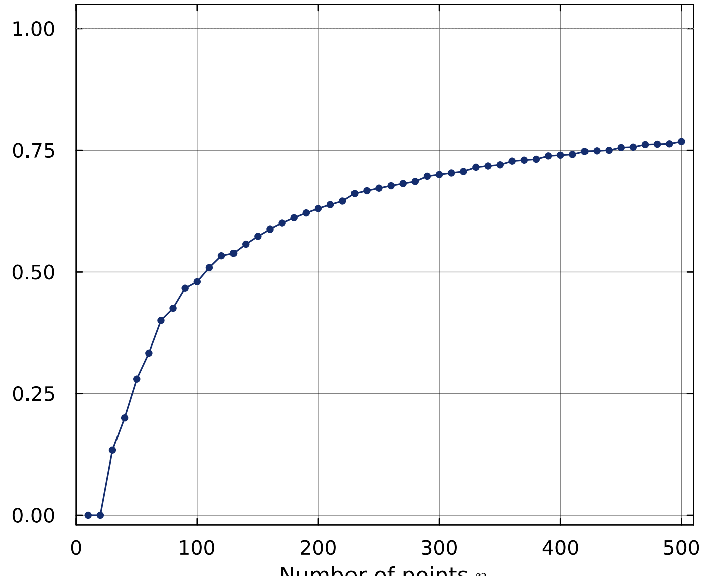
(b) Fraction of underflowed weights
