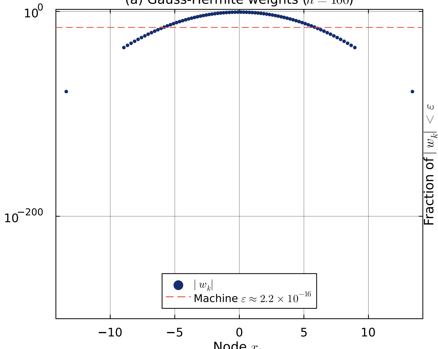
(a) Gauss-Hermite weights ( n = 100 )
