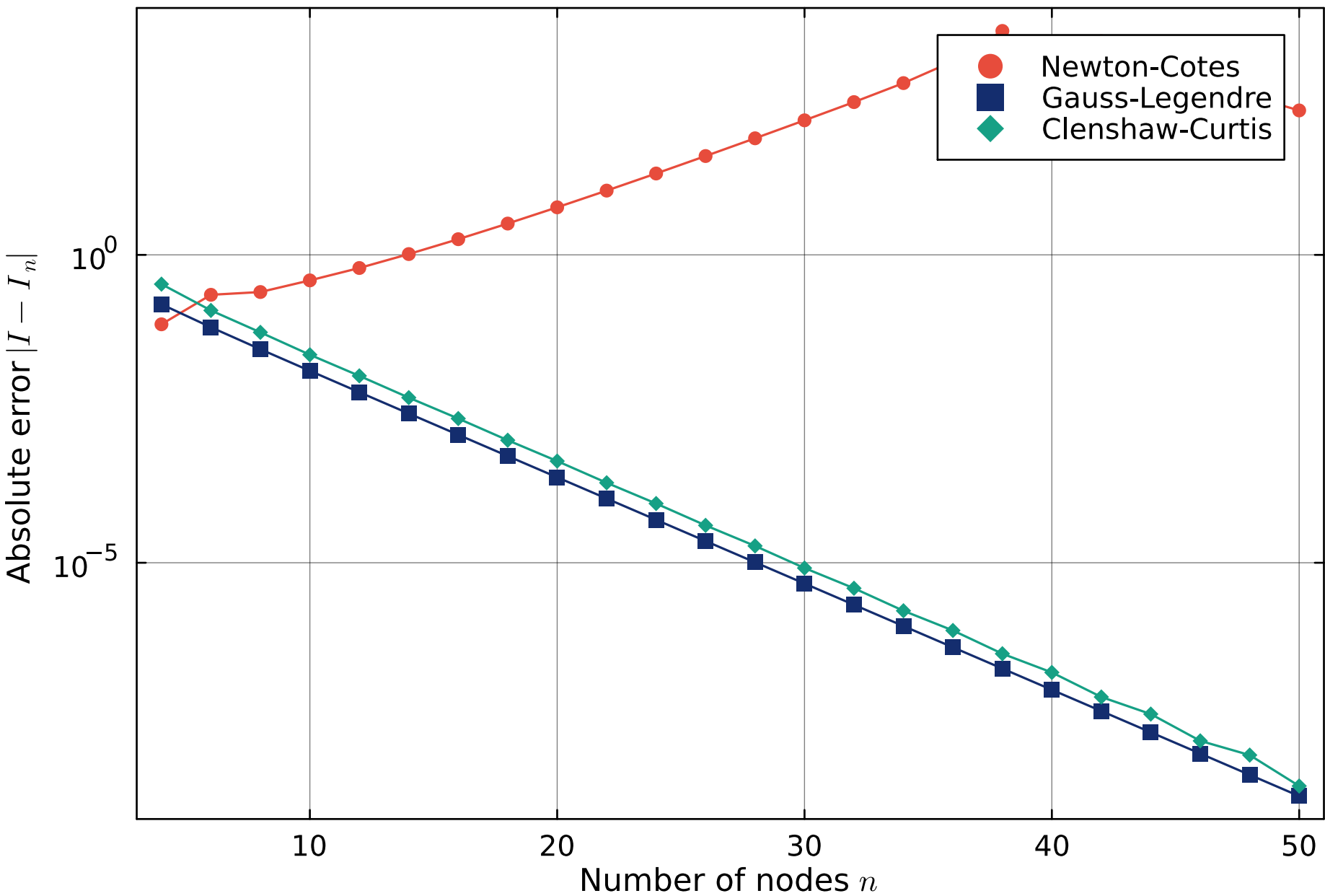
Quadrature of f(x) = 1/(1 + 25x^2) on [-1, 1]
