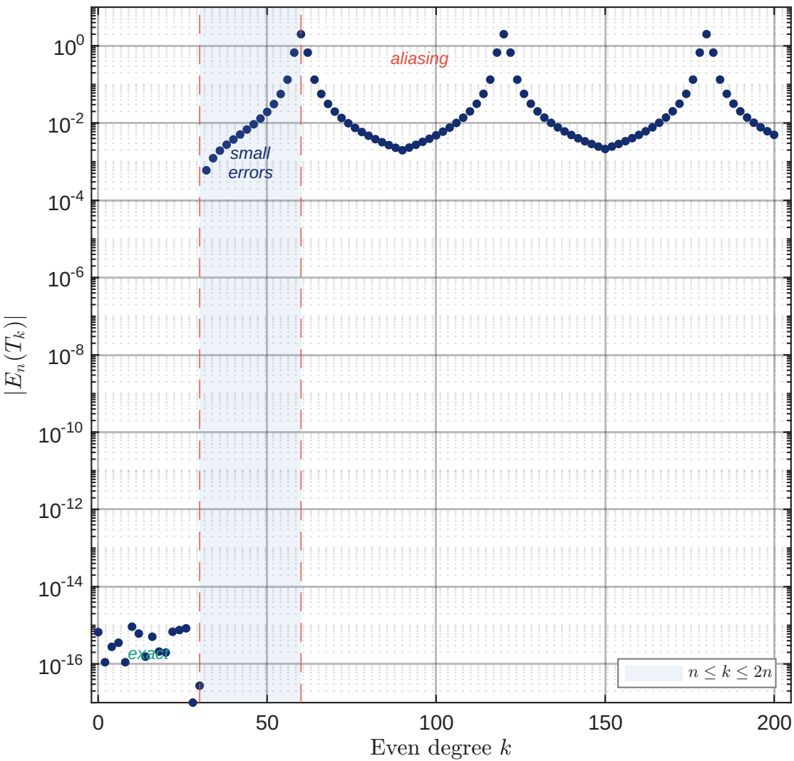
(a) CC error for Chebyshev polynomials ( n = 30 )
